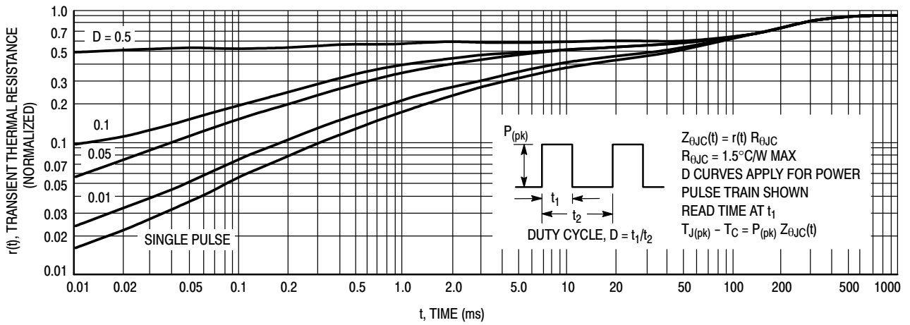
Figure 9. Thermal Response
