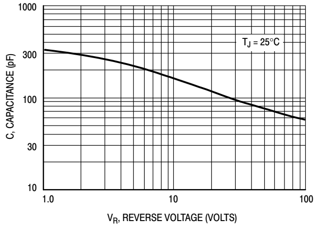
Figure 10. Typical Capacitance
