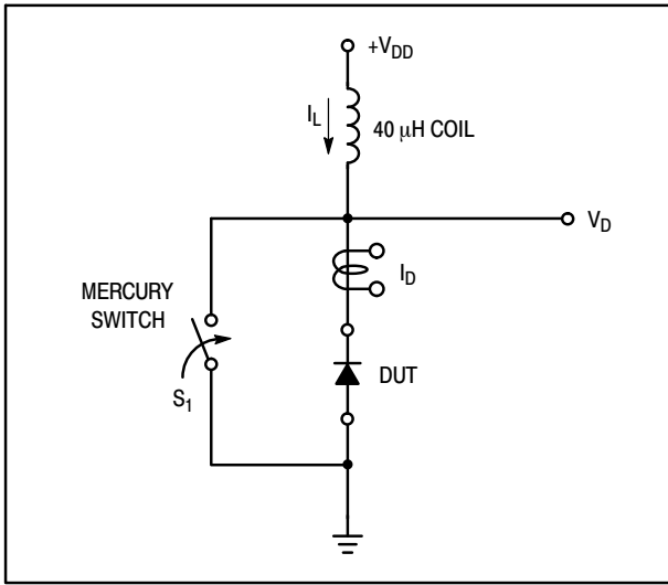
Figure 6. Test Circuit
