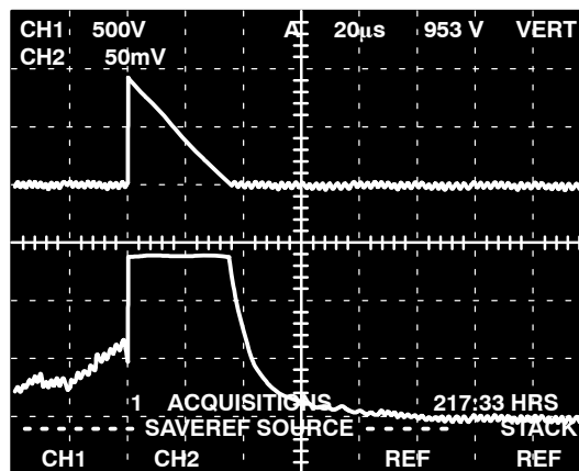
Figure 8. Current-Voltage Waveforms
