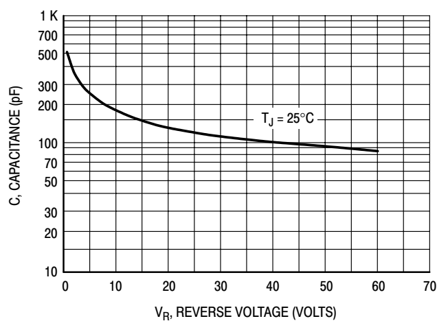
Figure 6. Typical Capacitance
