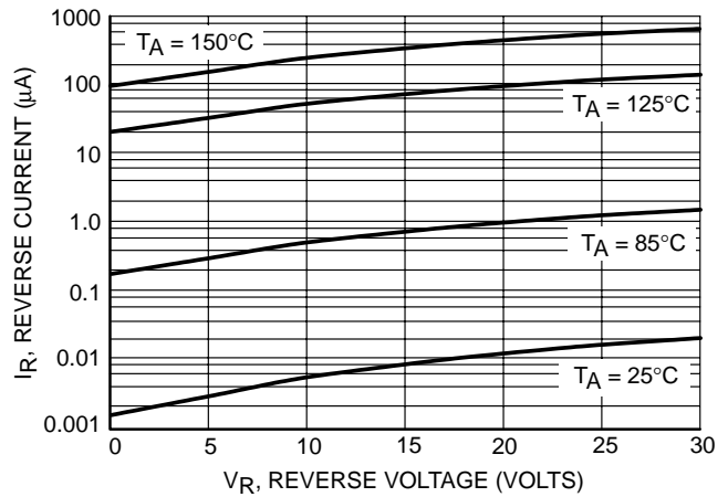
Figure 3. Leakage Current
