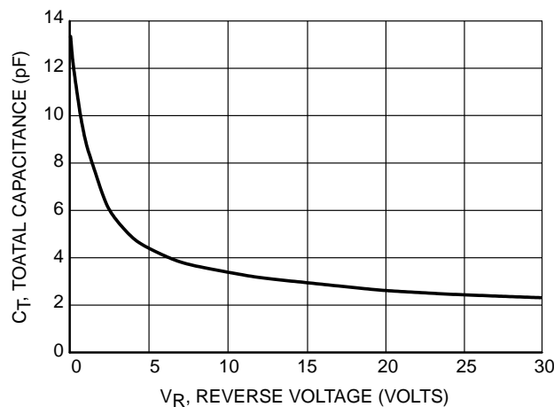
Figure 4. Total Capacitance
