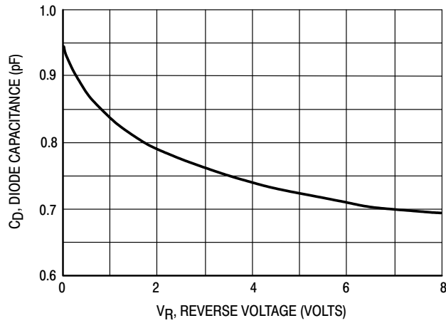
Figure 5. Capacitance
