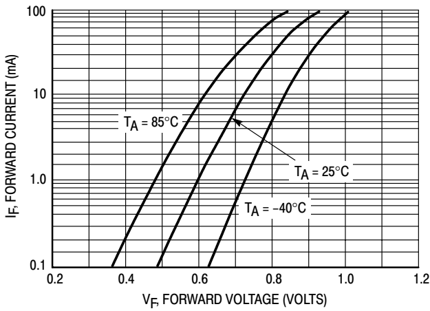
Figure 3. Forward Voltage
