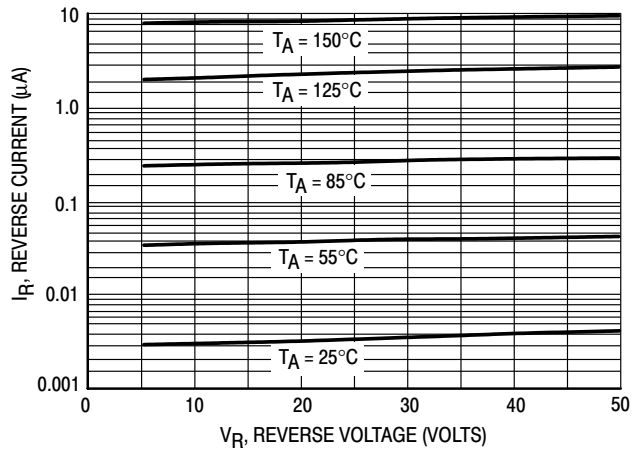
Figure 4. Leakage Current
