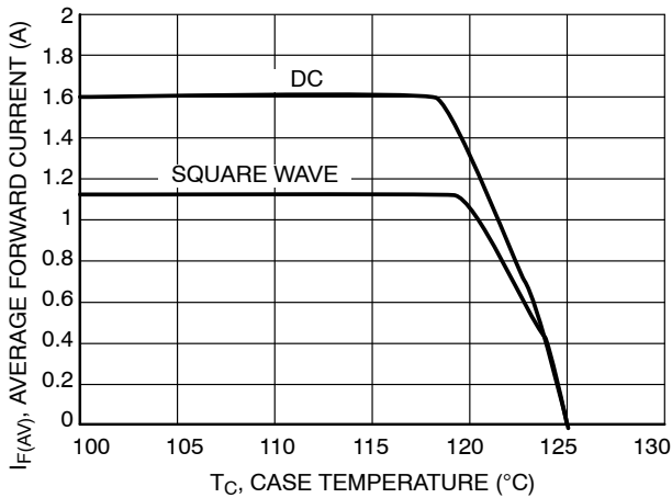
Figure 5. Current Derating (Case)
