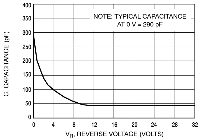
Figure 7. Typical Capacitance
