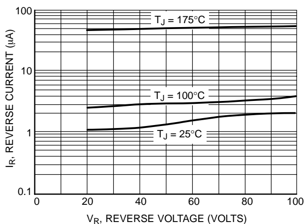
Figure 2. Maximum Reverse Current
