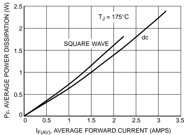
Figure 9. Power Dissipation
