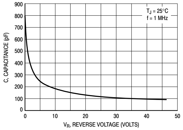
Figure 8. Typical Capacitance
