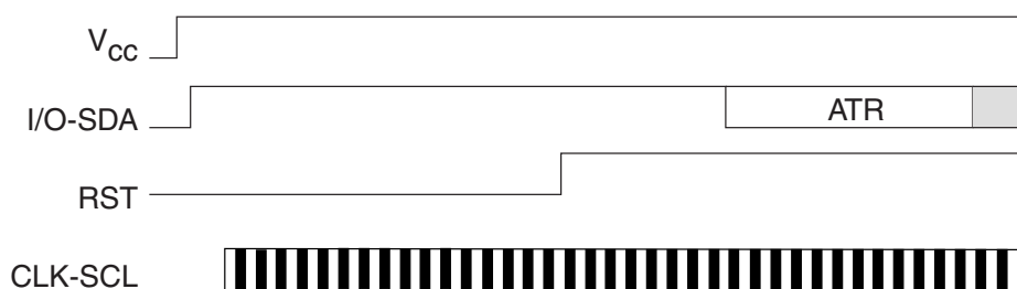
Figure 2. Asynchronous T = 0 Protocol (Gemplus Patent)
