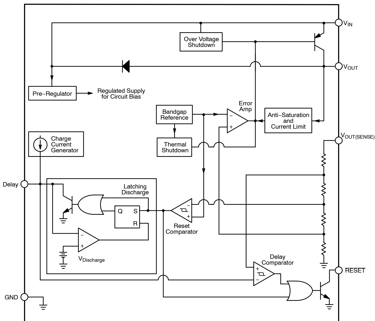
Figure 1. Block Diagram
