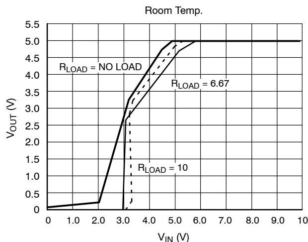
Figure 5. V_{OUT} vs. V_{IN} Over R_{LOAD}
