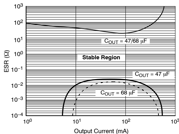
Figure 11. Output Capacitor ESR
