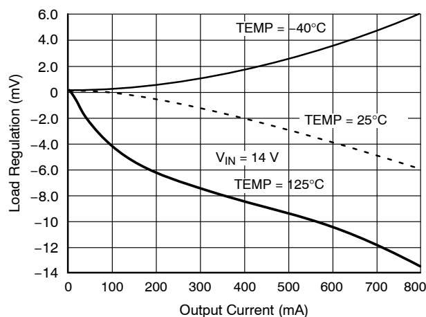
Figure 7. Load Regulation vs. Output Current Over Temperature
