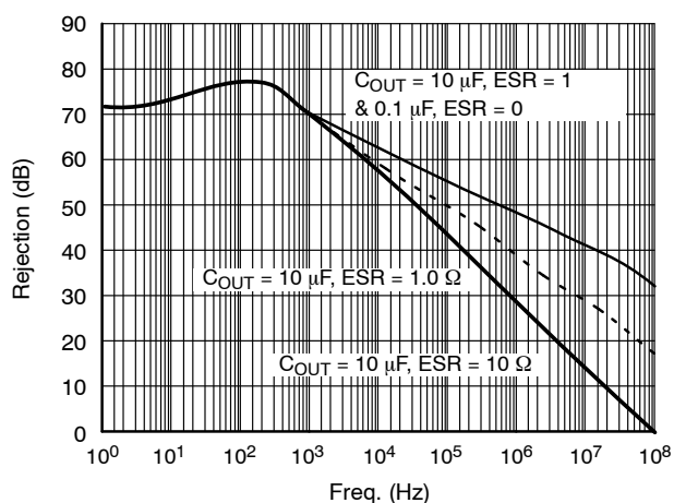
Figure 10. Ripple Rejection
