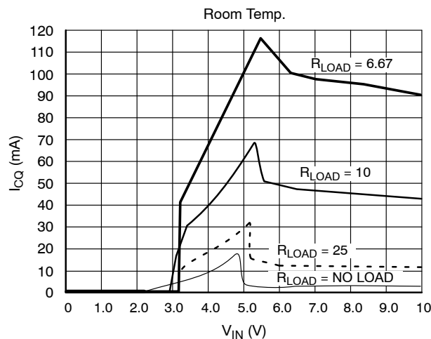
Figure 3. I_{CQ} vs. V_{IN} Over R_{LOAD}
