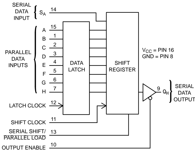
Figure 1. Logic Diagram
