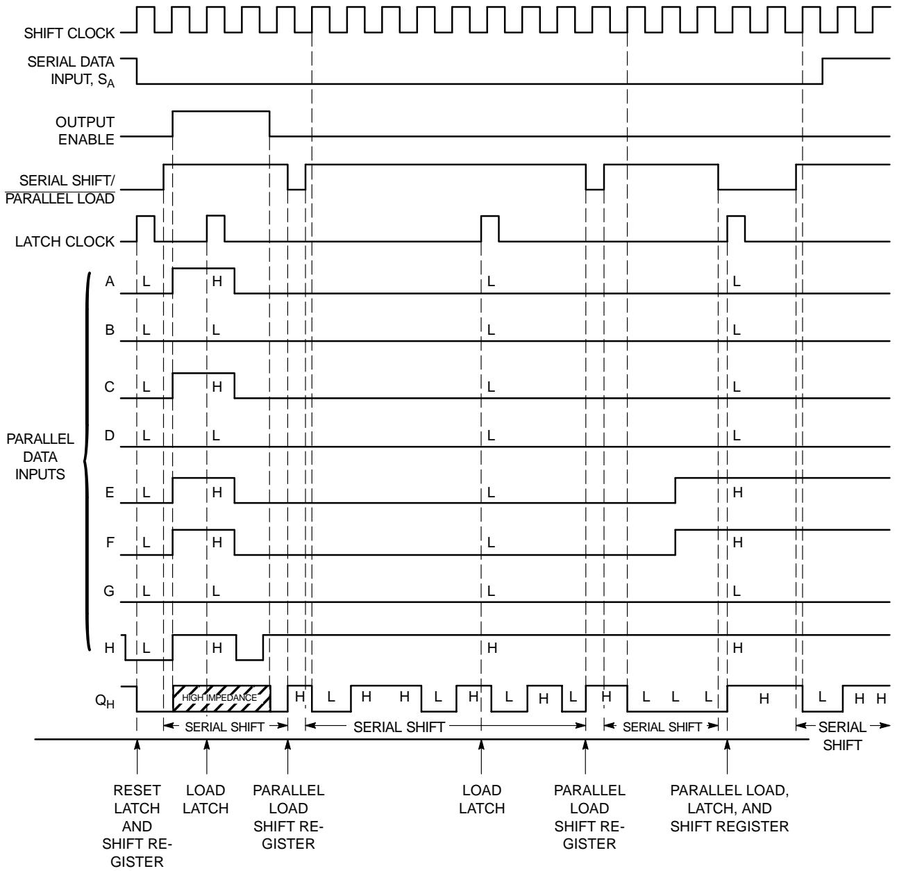
Figure 11. Timing Diagram
