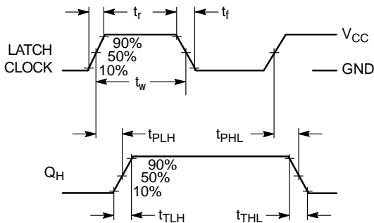
Figure 2. (Serial Shift/Parallel Load = L)
