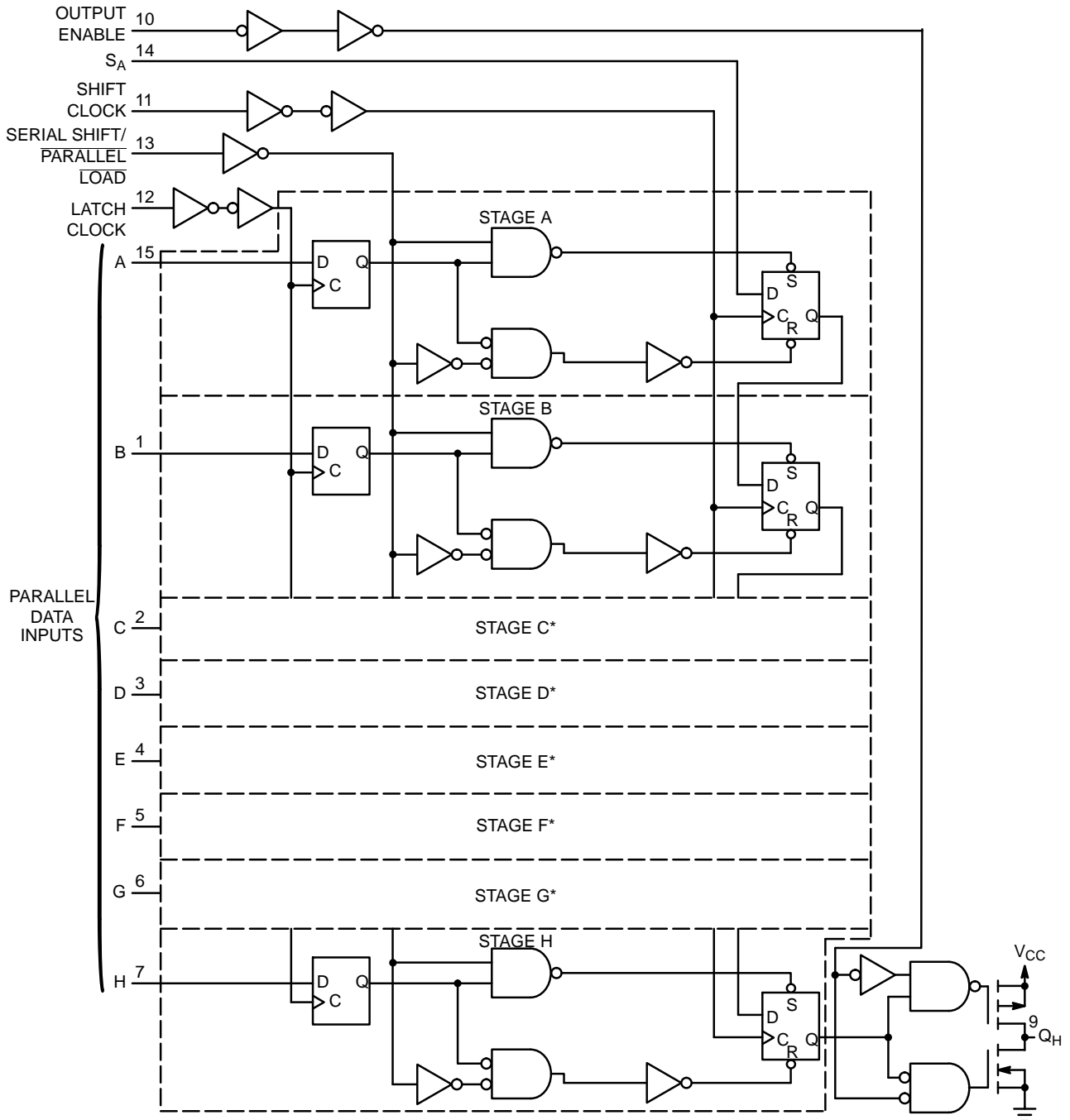
Figure 12. Logic Detail
