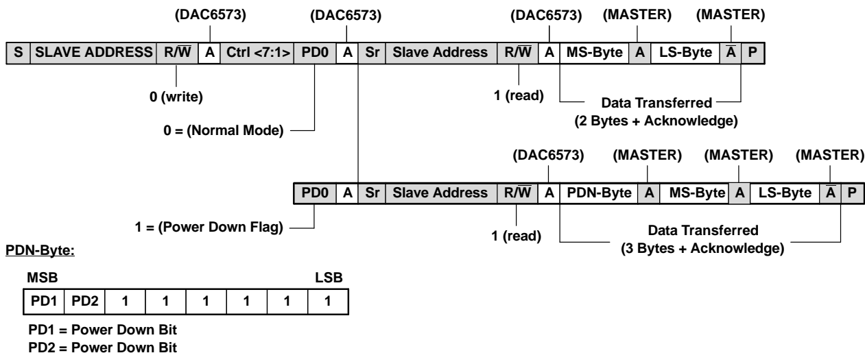
Figure 35. Standard and Fast Mode: Slave Transmitter
