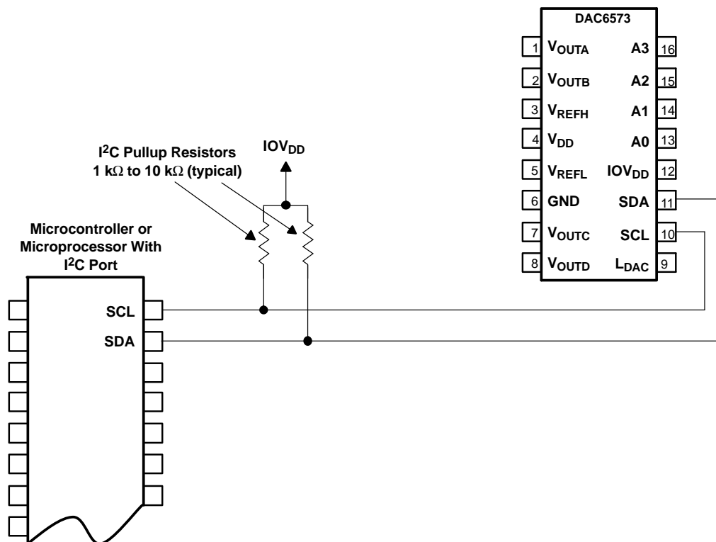
Figure 38. Typical DAC6573 Connections
