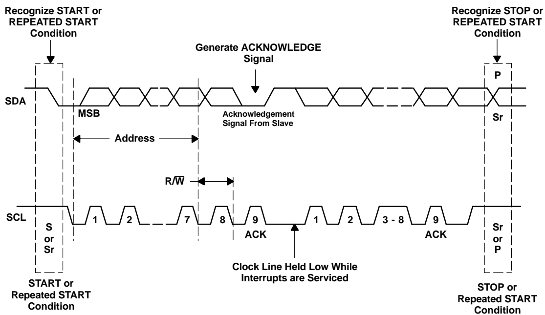
Figure 32. Bus Protocol
