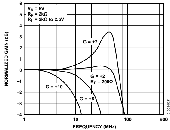
Figure 27. Closed-Loop Gain vs. Frequency Response
