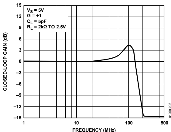
Figure 3. Frequency Response
