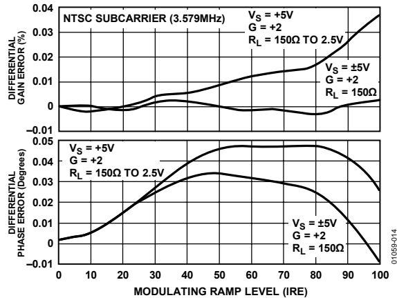
Figure 14. Differential Gain and Phase Errors
