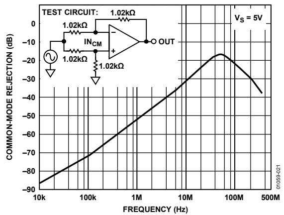
Figure 21. Common-Mode Rejection vs. Frequency
