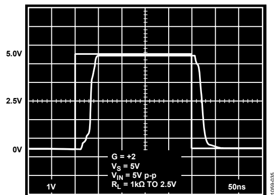
Figure 37. Overdrive Recovery
