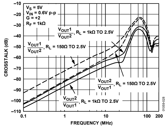
Figure 28. Crosstalk (Output-to-Output) vs. Frequency
