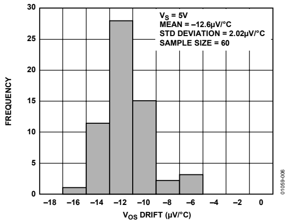
Figure 6. V_{OS} Drift Over -40^{\circ}\text{C} to +85^{\circ}\text{C}
