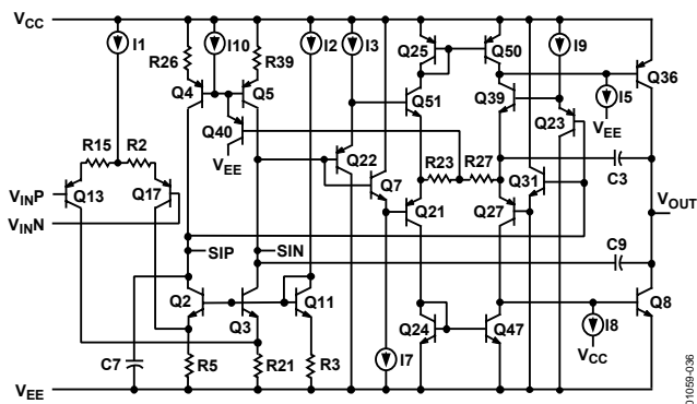
Figure 35. Simplified Schematic
