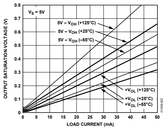
Figure 22. Output Saturation Voltage vs. Load Current
