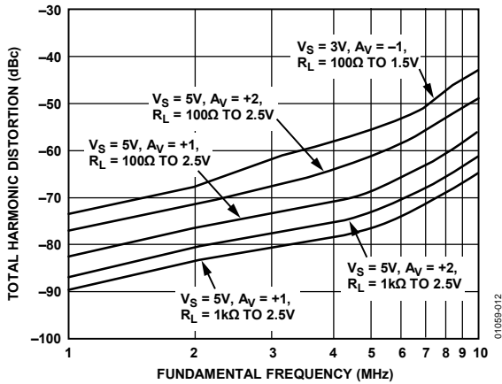
Figure 12. Total Harmonic Distortion vs. Frequency
