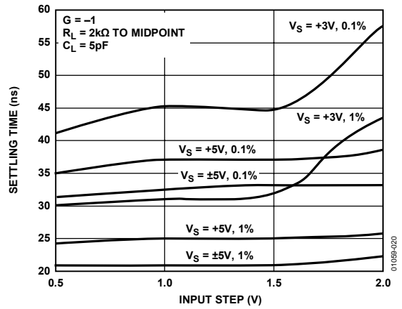
Figure 20. Settling Time vs. Input Voltage
