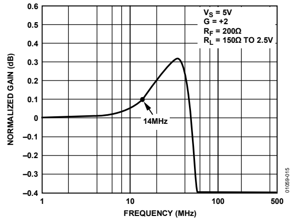
Figure 15. 0.1 dB Gain Flatness
