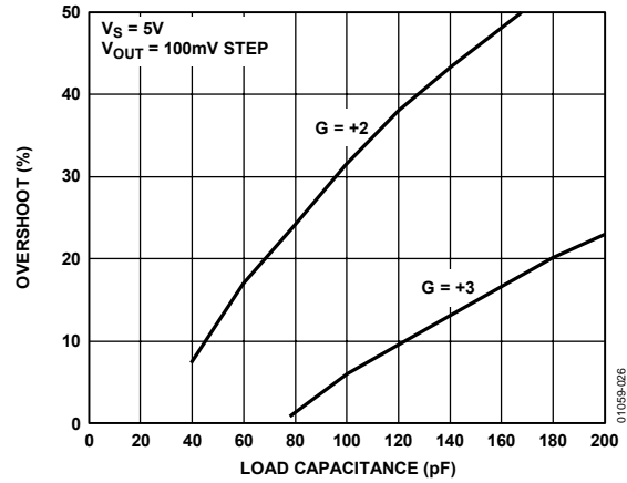
Figure 26. Overshoot vs. Load Capacitance
