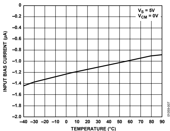
Figure 7. I_b vs. Temperature
