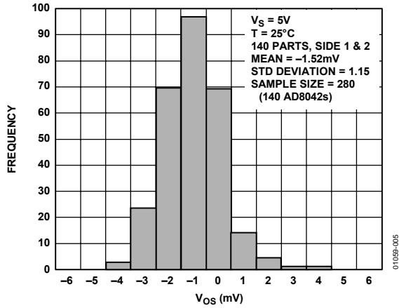
Figure 5. Typical Distribution of V_{OS}
