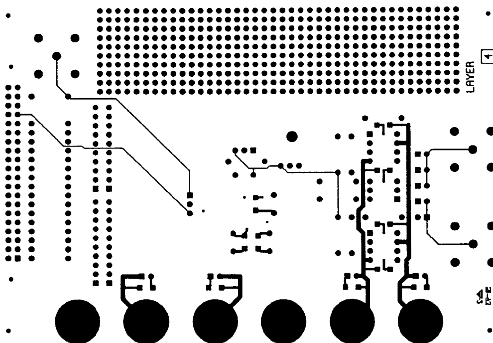
Figure 37. Component Side PCB Layout (Not to Scale)
