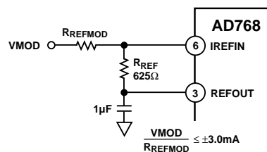
Figure 31. Typical Multiplying DAC Application
