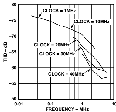
Figure 19. THD vs. F_{OUT}
