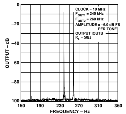
Figure 20. Intermodulation Distortion
