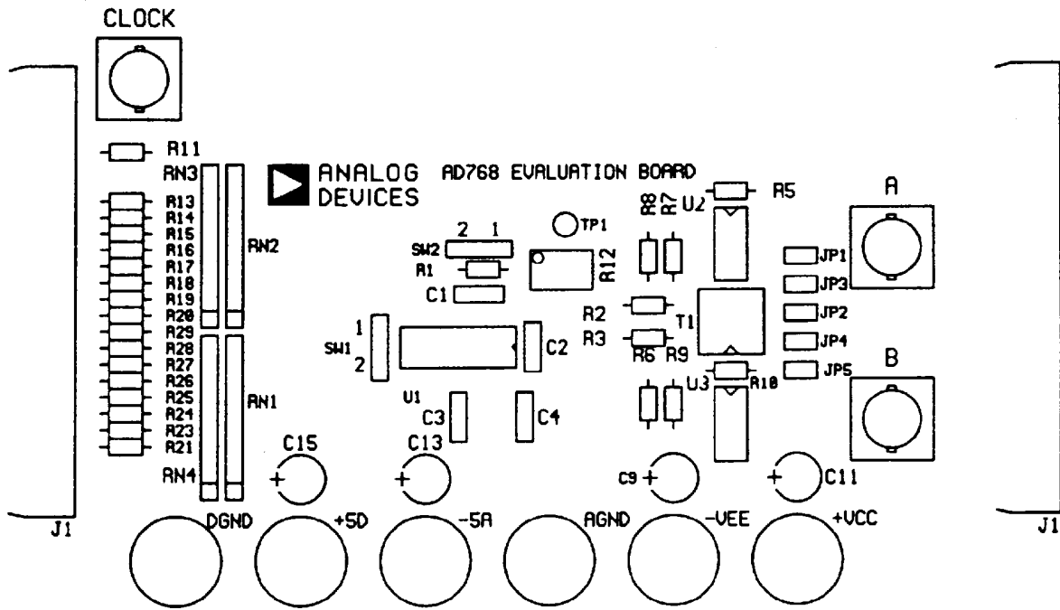
Figure 36. Silkscreen Layer (Not to Scale)
