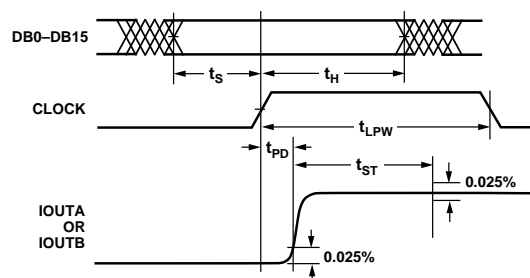
Timing Diagram
