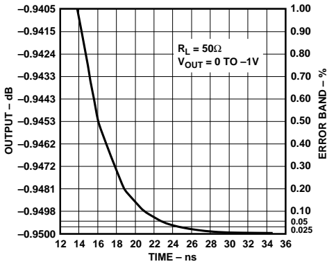
Figure 12. Settling Time
