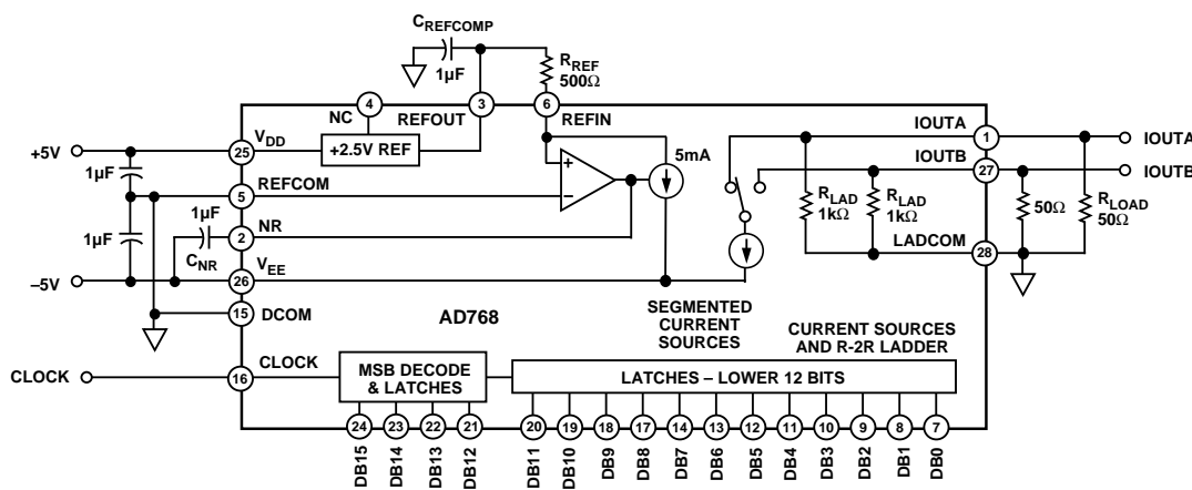
Figure 1. Functional Block Diagram and Basic Hookup
