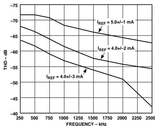
Figure 32. Reference Channel Distortion vs. Frequency
