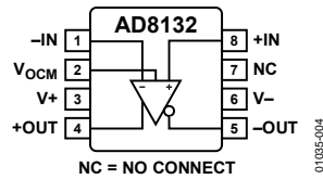
Figure 4. Pin Configuration
