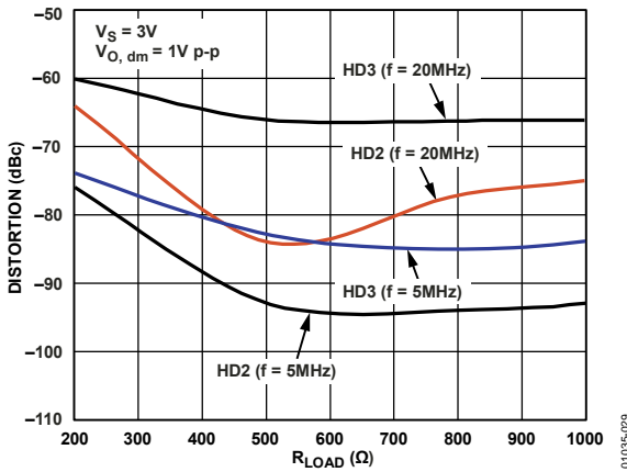
Figure 24. Harmonic Distortion vs. R_{LOAD} , G = +1 (See Figure 62)
