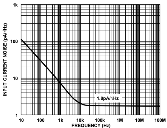
Figure 52. Input Current Noise vs. Frequency
