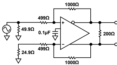
Figure 57. Basic Test Circuit, G = +2
