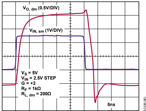
Figure 53. Overdrive Recovery
