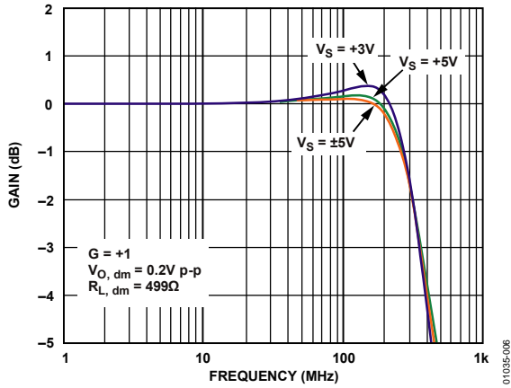
Figure 5. Small Signal Frequency Response (See Figure 56)
