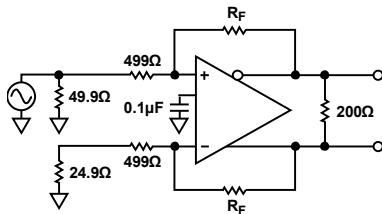
Figure 58. Test Circuit for Various Gains
