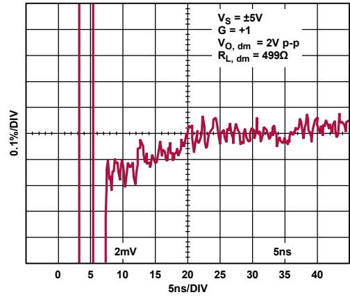
Figure 44. 0.1% Settling Time
