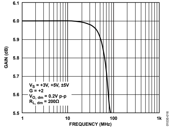
Figure 14. 0.1 dB Flatness vs. Frequency (See Figure 57)
