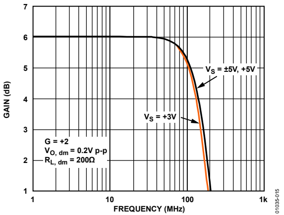
Figure 13. Small Signal Frequency Response (See Figure 57)
