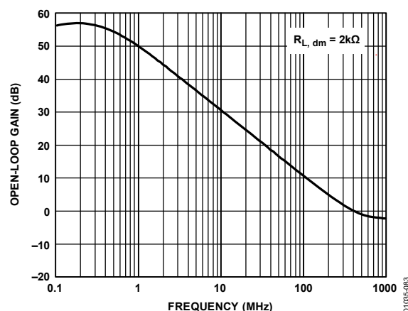
Figure 65. Open-Loop Gain vs. Frequency
