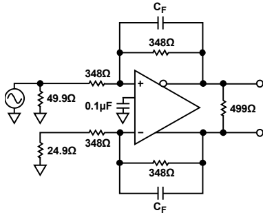
Figure 56. Basic Test Circuit, G = +1
