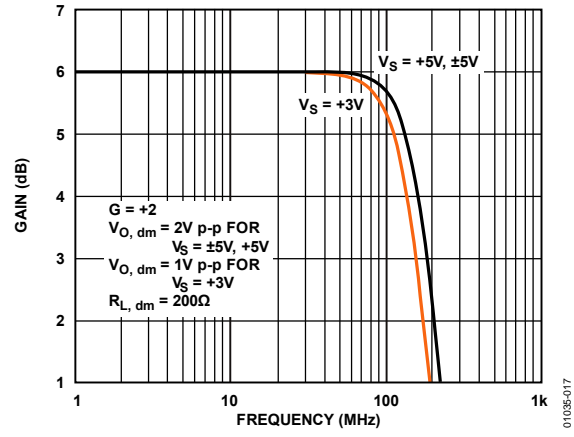
Figure 15. Large Signal Frequency Response (See Figure 57)
