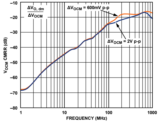
Figure 50. V_{OCM} CMRR vs. Frequency
