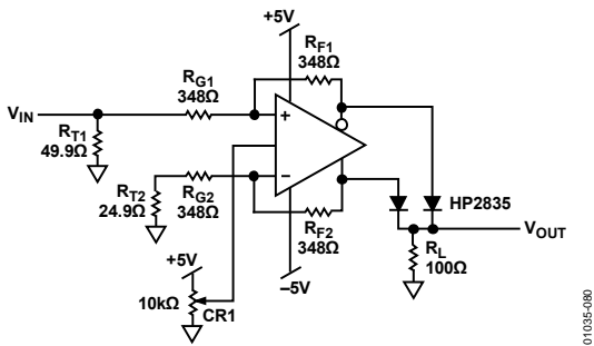
Figure 82. Full-Wave Rectifier
