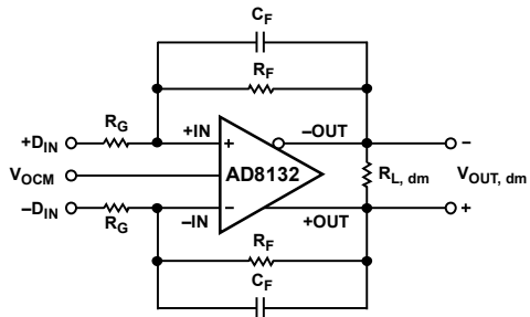
Figure 64. Circuit Definitions
