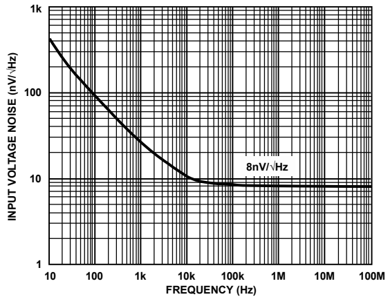
Figure 51. Input Voltage Noise vs. Frequency
