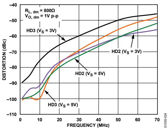
Figure 19. Harmonic Distortion vs. Frequency, G = +1 (See Figure 62)
