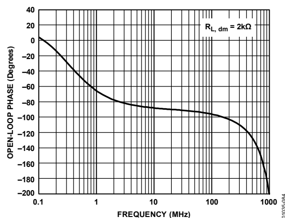
Figure 66. Open-Loop Phase vs. Frequency
