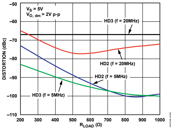
Figure 25. Harmonic Distortion vs. R_{LOAD} , G = +1 (See Figure 62)
