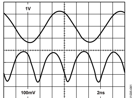
Figure 83. Full-Wave Rectifier Response with 100 MHz Input
