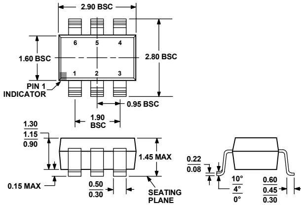
Figure 35. 6-Lead Small Outline Transistor Package [SOT-23] (RT-6) Dimensions shown in millimeters
