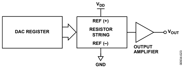
Figure 23. DAC Architecture
