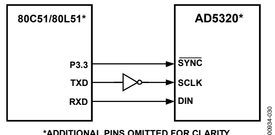
Figure 30. AD5320 to 80C51/80L51 Interface
