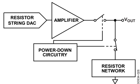
Figure 27. Output Stage During Power-Down
