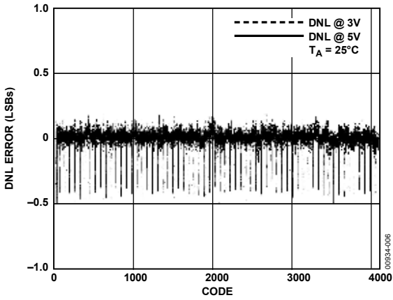
Figure 6. Typical DNL Plot
