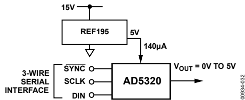
Figure 32. REF195 as Power Supply to AD5320
