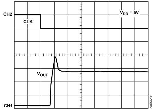
CH1 1V, CH2 5V, TIME BASE = 5µs/DIV
