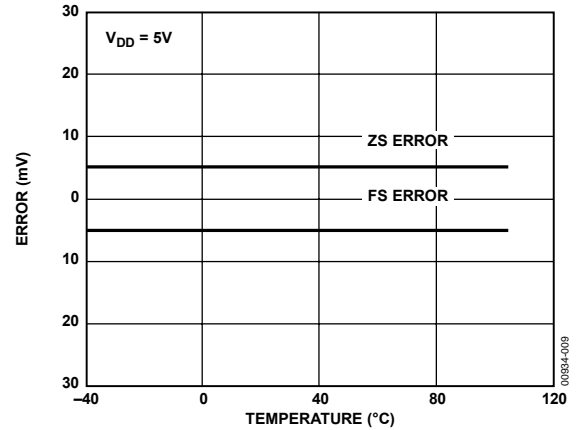
Figure 9. Zero-Scale Error and Full-Scale Error vs. Temperature
