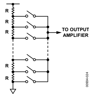
Figure 24. Resistor String
