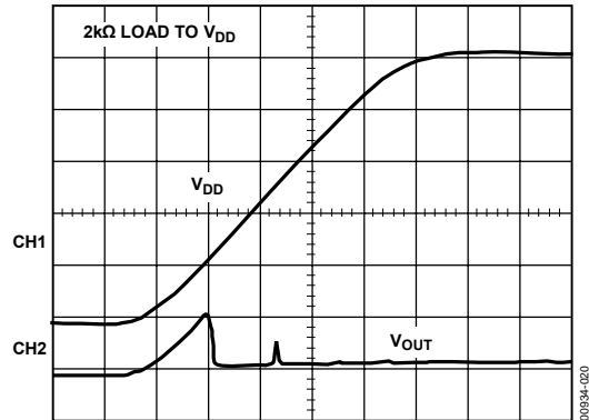
CH1 1V, CH2 1V, TIME BASE = 20µs/DIV
