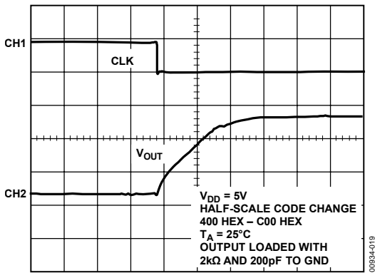
CH1 1V, CH2 5V, TIME BASE = 1µs/DIV
