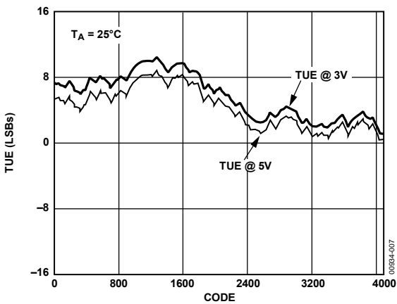
Figure 7. Typical Total Unadjusted Error Plot
