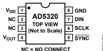
Figure 4. MSOP Pin Configuration
