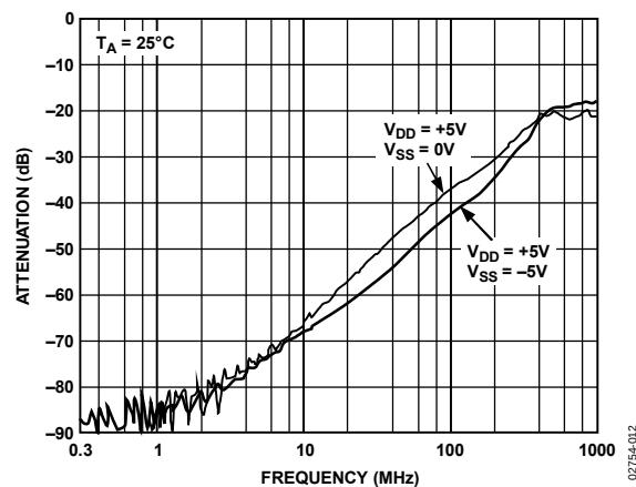
Figure 12. Crosstalk vs. Frequency
