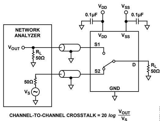
Figure 23. Channel-to-Channel Crosstalk
