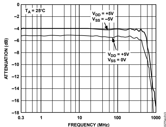
Figure 13. On Response vs. Frequency
