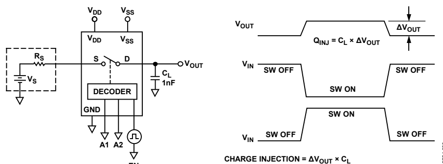
Figure 20. Charge Injection
