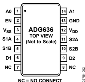
Figure 2. Pin Configuration
