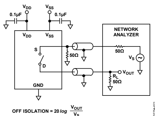
Figure 21. Off Isolation
