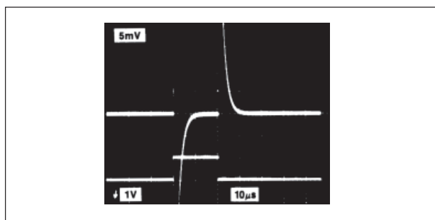
FIGURE 2C: Pulse Response with Output Decoupling
