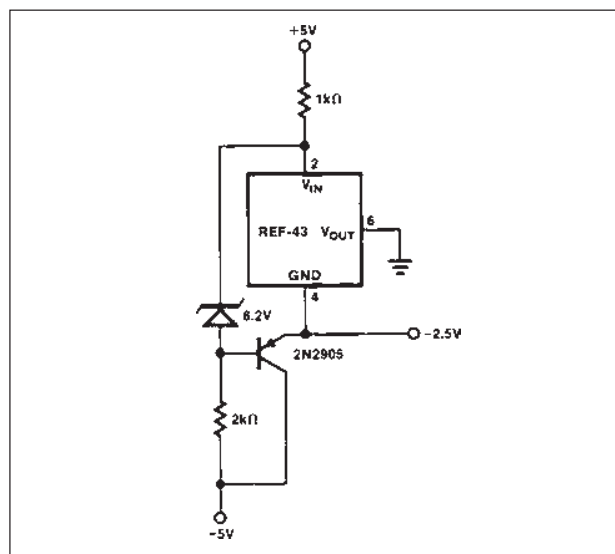
FIGURE 4: -2.5V Reference
