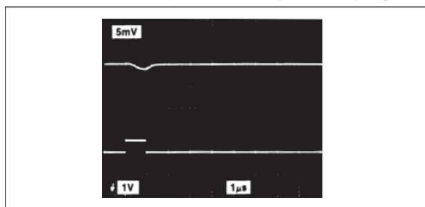
FIGURE 2C: Pulse Response with Output Decoupling
