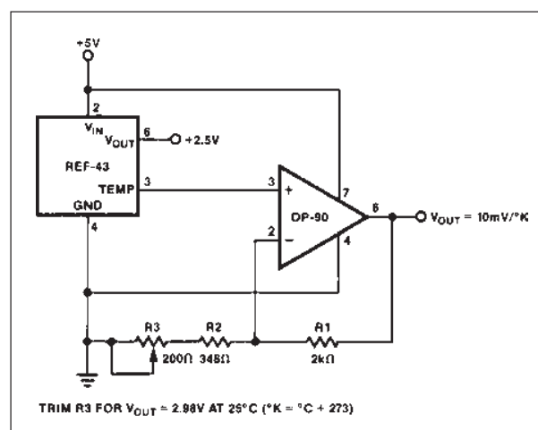
FIGURE 8: Single-Supply Kelvin-Output Thermometer
