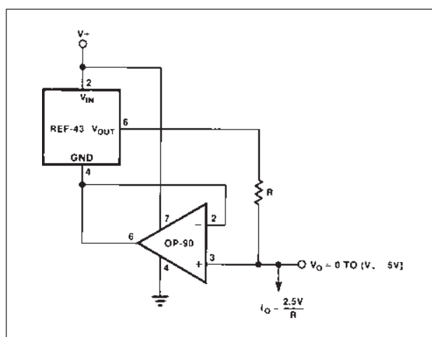
FIGURE 7: Precision Current Source
