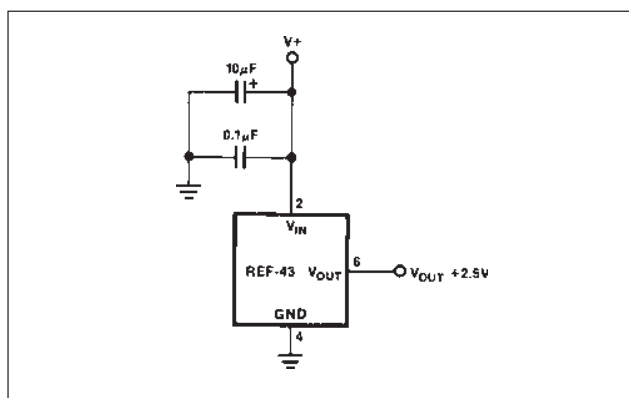
FIGURE 1: Basic Connections
