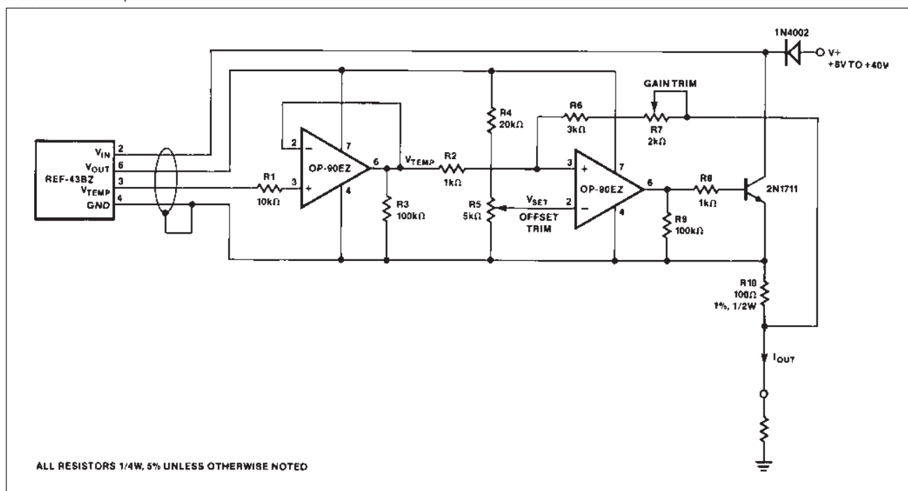
FIGURE 11: Temperature to 4-20mA Transmitter
