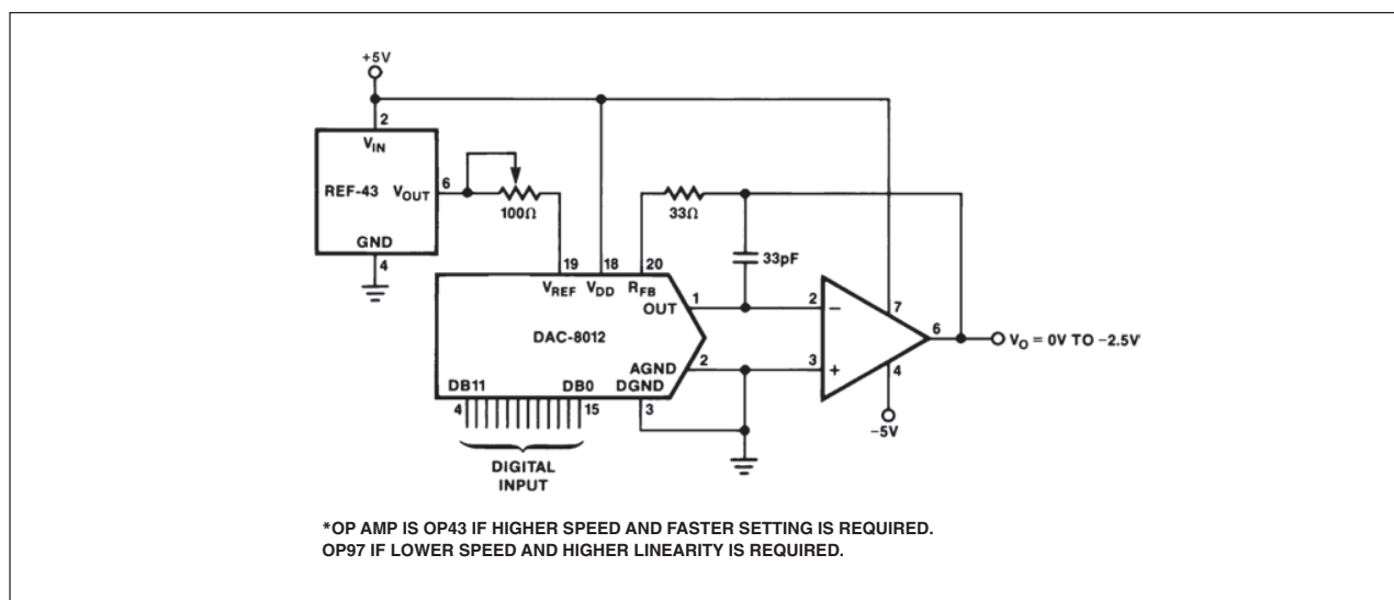
FIGURE 6: CMOS DAC Reference
