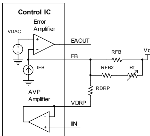
Figure 9. Temperature compensation of inductor DCR
