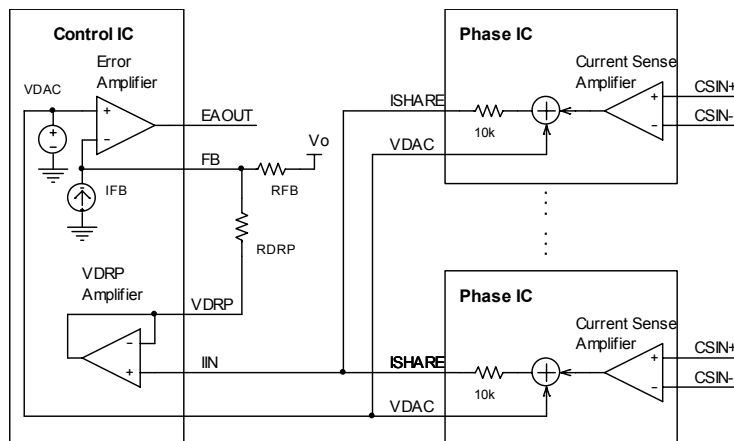
Figure 8. Adaptive voltage positioning
