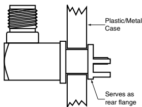
MOUNTING METHOD
