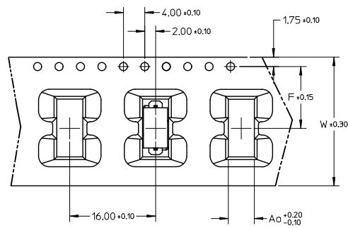
EMBOSSED TYPE B
