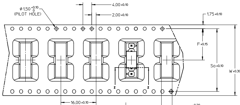
EMBOSSED TYPE A
