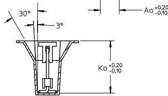
SECTION Z-Z
