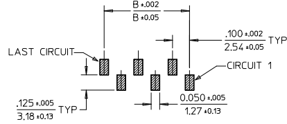
PCB LAYOUT: COMPONENT SIDE
