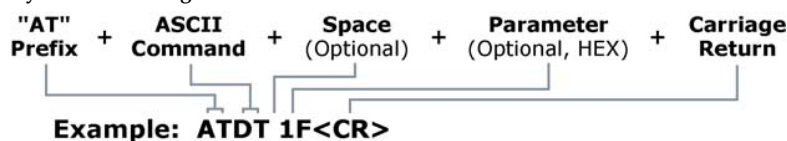
Figure 2-08. Syntax for sending AT Commands
