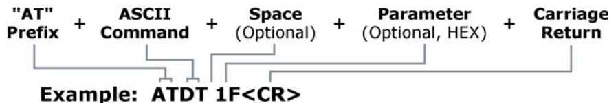
Figure B-2. Syntax for sending AT Commands
