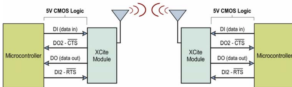
Figure 2-01. Data Flow in a UART-interfaced environment
