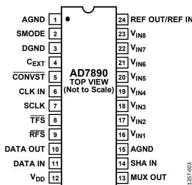
Figure 3. Pin Configuration
