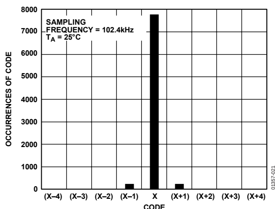
Figure 21. Histogram of 8192 Conversions with Write During Conversion
