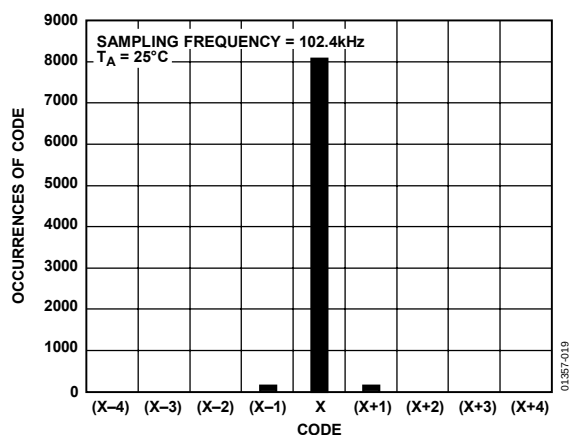
Figure 19. Histogram of 8192 Conversions of a DC Input
