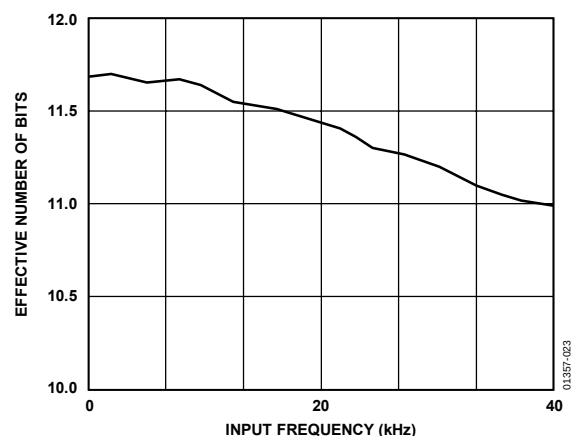
Figure 23. Effective Number of Bits vs. Frequency
