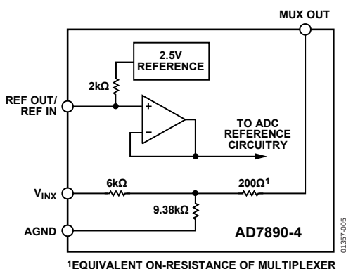
Figure 5. AD7890-4 Analog Input Structure
