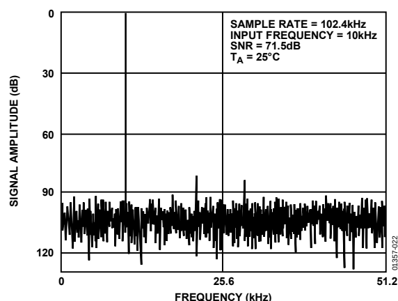
Figure 22. AD7890 FFT Plot
