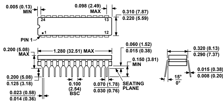
Figure 25. 24-Lead Ceramic Dual In-Line Package [CERDIP] (Q-24)
