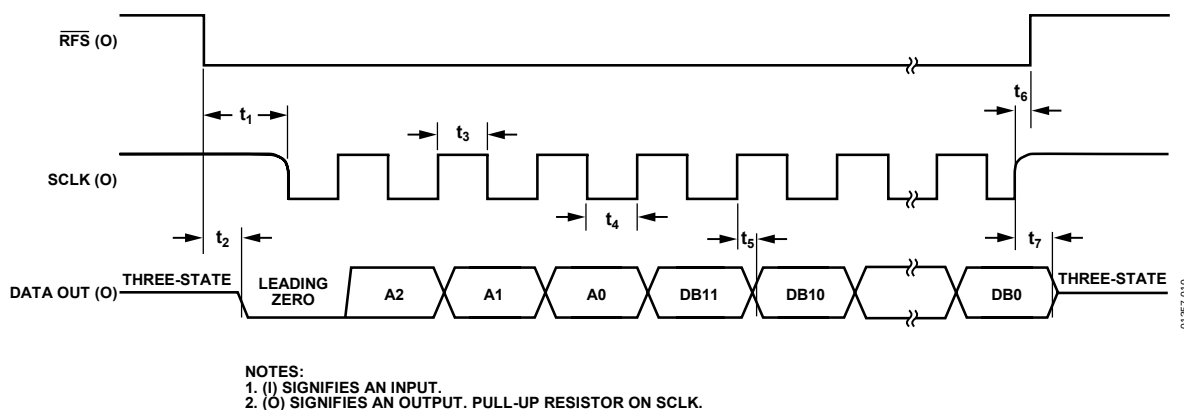
Figure 10. Self-Clocking (Master) Mode Output Register Read
