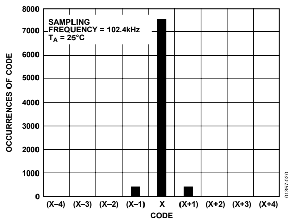
Figure 20. Histogram of 8192 Conversions with Read During Conversion
