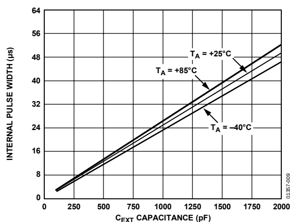
Figure 9. Internal Pulse Width vs. C EXT
