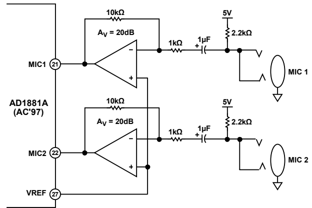
Figure 32. Microphone Preamplifier
