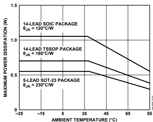
Figure 27. Maximum Power Dissipation vs. Temperature (5-Lead and 14-Lead Package Types)
