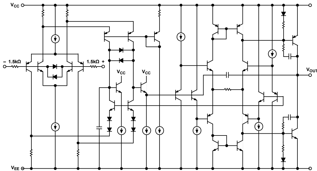
Figure 26. Simplified Schematic
