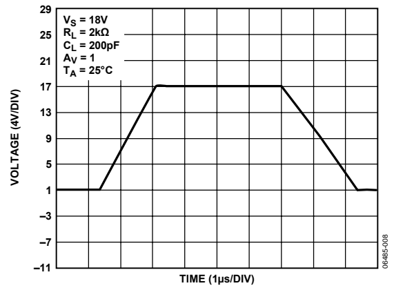
Figure 8. Large Signal Transient Response, V_S = 18V
