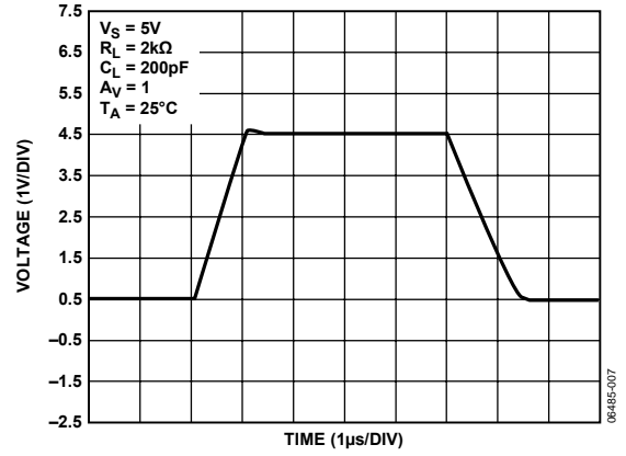
Figure 7. Large Signal Transient Response, V_S = 5V
