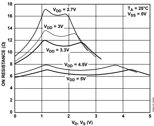
Figure 5. On Resistance vs. V_D , V_S (Single Supply)
