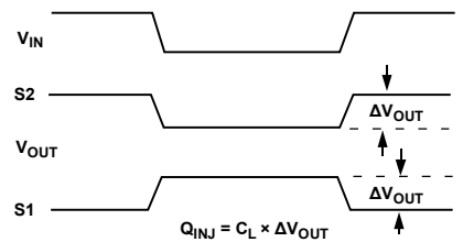
Figure 21. Charge Injection
