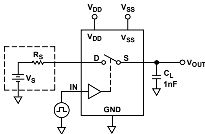
Figure 21. Charge Injection
