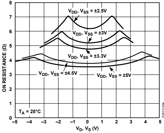
Figure 4. On Resistance vs. V_D , V_S (Dual Supply)
