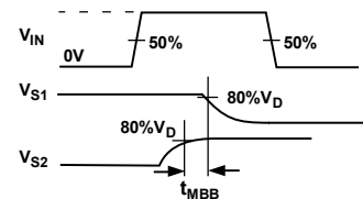
Figure 20. Make-Before-Break Time Delay, t_{MBS} (ADG620 Only)
