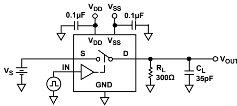
Figure 18. Switching Times
