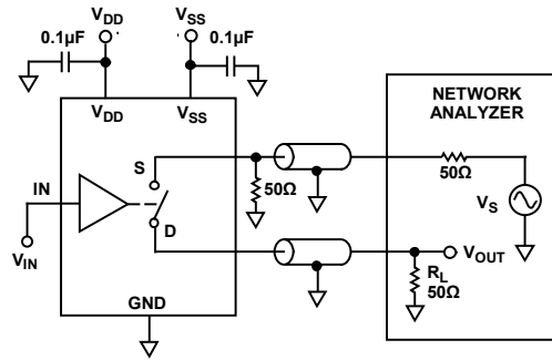
Figure 22. Off Isolation
