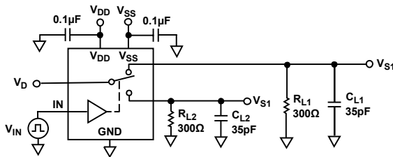
Figure 19. Break-Before-Make Time Delay, t_{BBM} (ADG619 Only)
