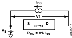
Figure 15. On Resistance
