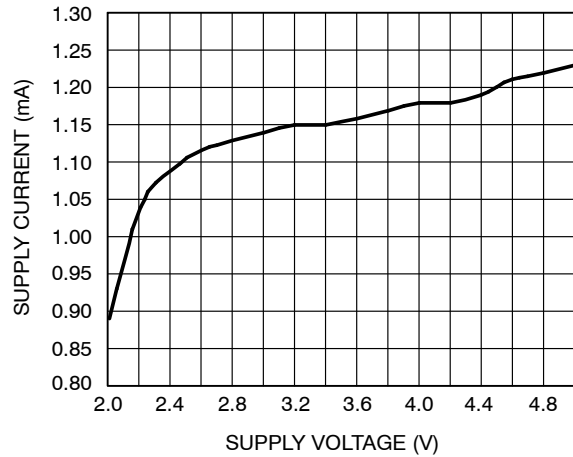
Figure 12. Supply Current vs. Supply Voltage
