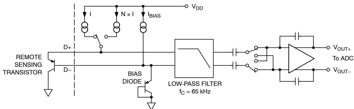
Figure 18. Signal Conditioning
