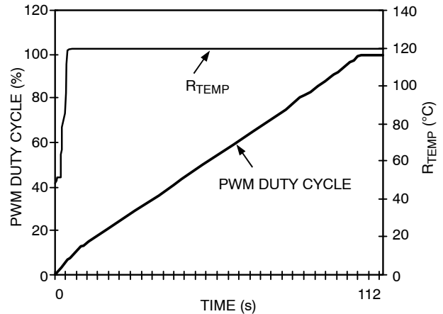
Figure 32. Filtered Mode with Ramp Rate = 1
