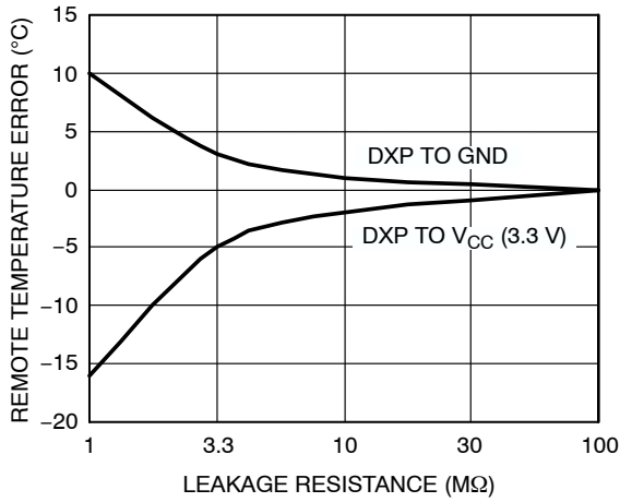
Figure 3. Temperature Error vs. PCB Track Resistance
