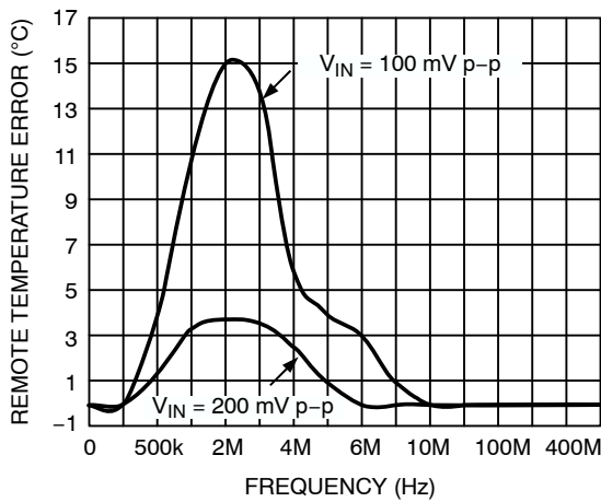
Figure 5. Temperature Error vs. Power Supply Noise Frequency
