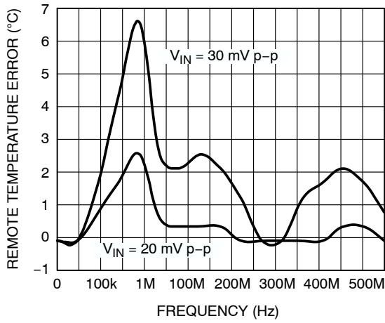
Figure 9. Temperature Error vs. Differential-mode Noise Frequency
