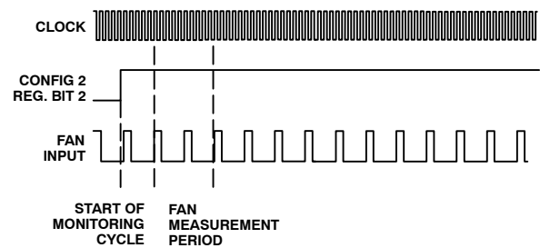
Figure 37. Fan Speed Measurement
