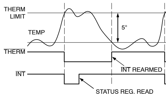
Figure 20. Operation of \overline{\text{THERM}} and \overline{\text{INT}} Signals
