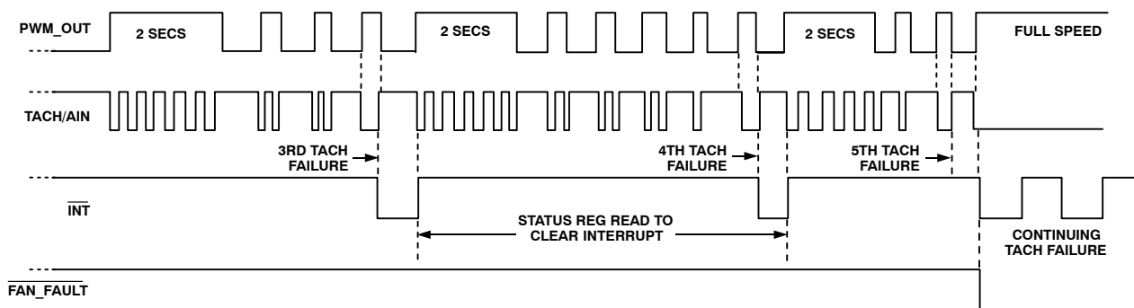
Figure 38. Operation of \overline{\text{FAN\_FAULT}} and Interrupt Pins
