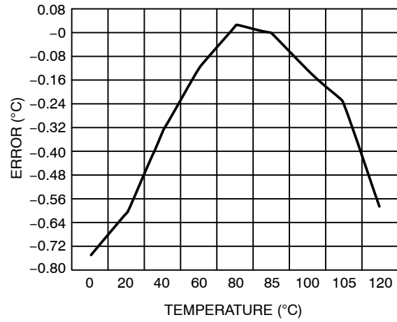
Figure 10. Remote Sensor Error
