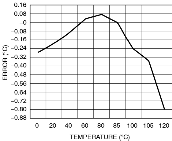
Figure 13. Local Sensor Error
