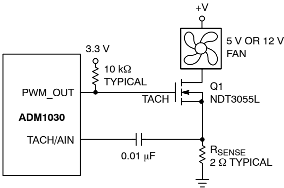
Figure 35. Interfacing the ADM1030 to a 2-wire Fan
