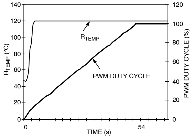
Figure 31. Filtered Mode with Ramp Rate = 2
