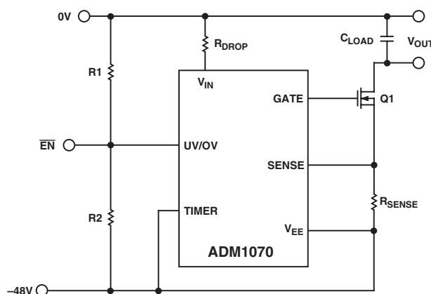
Figure 15. UV/OV Used as Enable Input
