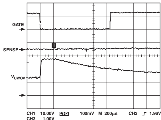
Figure 7. Timing Waveforms Associated with an Overvoltage Glitch
