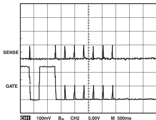
Figure 13. Illustration of the PWM Ratio ( t_{ON}/t_{OFF} )
