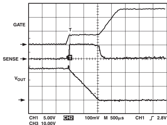
Figure 6. Start-Up Sequence
