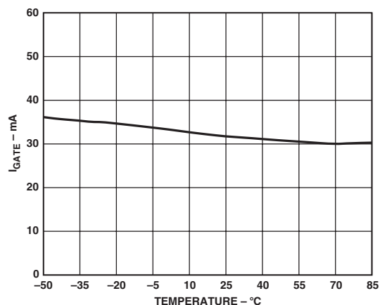
TPC 10. I_{GATE} (FCL, Sink) vs. Temperature ( V_{GATE} = 9\text{ V} )
