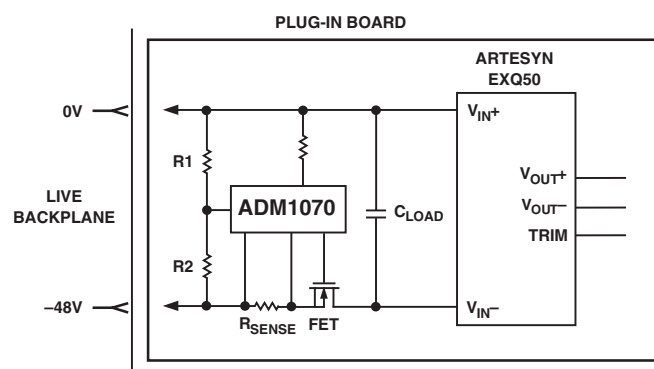
Figure 1. Topology
