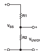
Figure 3. Voltage Divider
