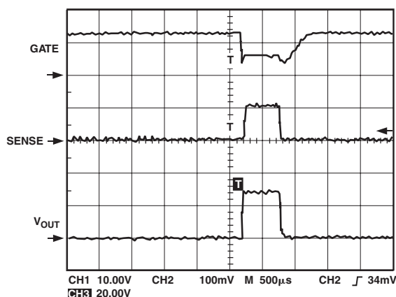
Figure 9. Timing Waveforms Associated with a Current Glitch
