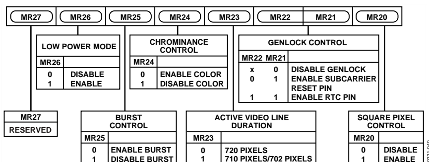
Figure 40. Mode Register 2
