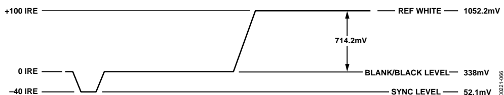
Figure 66. NTSC Luma Video Levels
