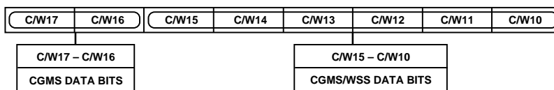
Figure 52. CGMS_WSS Register 1
