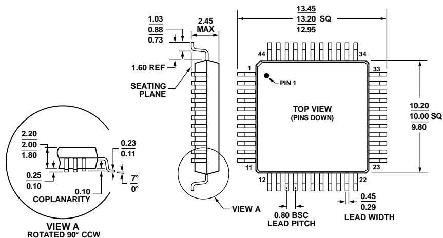
COMPLIANT TO JEDEC STANDARDS MS-022-AB-1 Figure 105. 44-Lead Metric Quad Flat Package [MQFP] (S-44-1)
