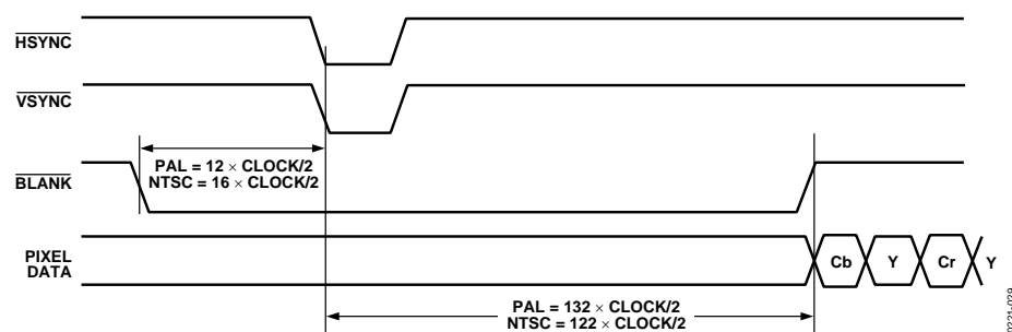
Figure 29. Timing Mode 2 Even-to-Odd Field Transition Master/Slave
