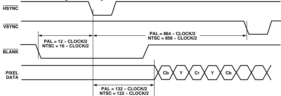
Figure 30. Timing Mode 2 Odd-to-Even Field Transition Master/Slave
