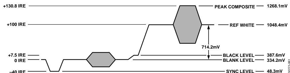
Figure 61. NTSC Composite Video Levels
