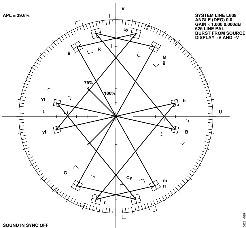
Figure 89. PAL Vector Plot
