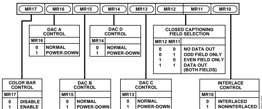
Figure 39. Mode Register 1
