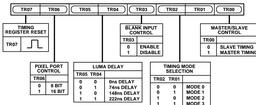
Figure 43. Timing Register 0
