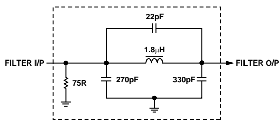
Figure 79. Output Filter
