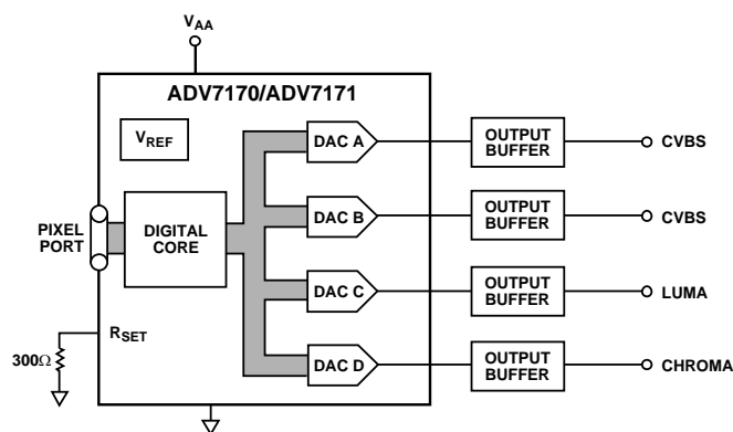
Figure 81. Output DAC Buffering Configuration
