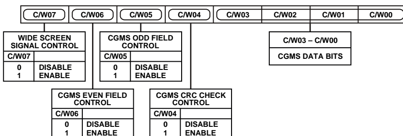
Figure 51. CGMS_WSS Register 0
