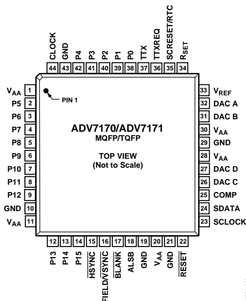
Figure 5. Pin Configuration
