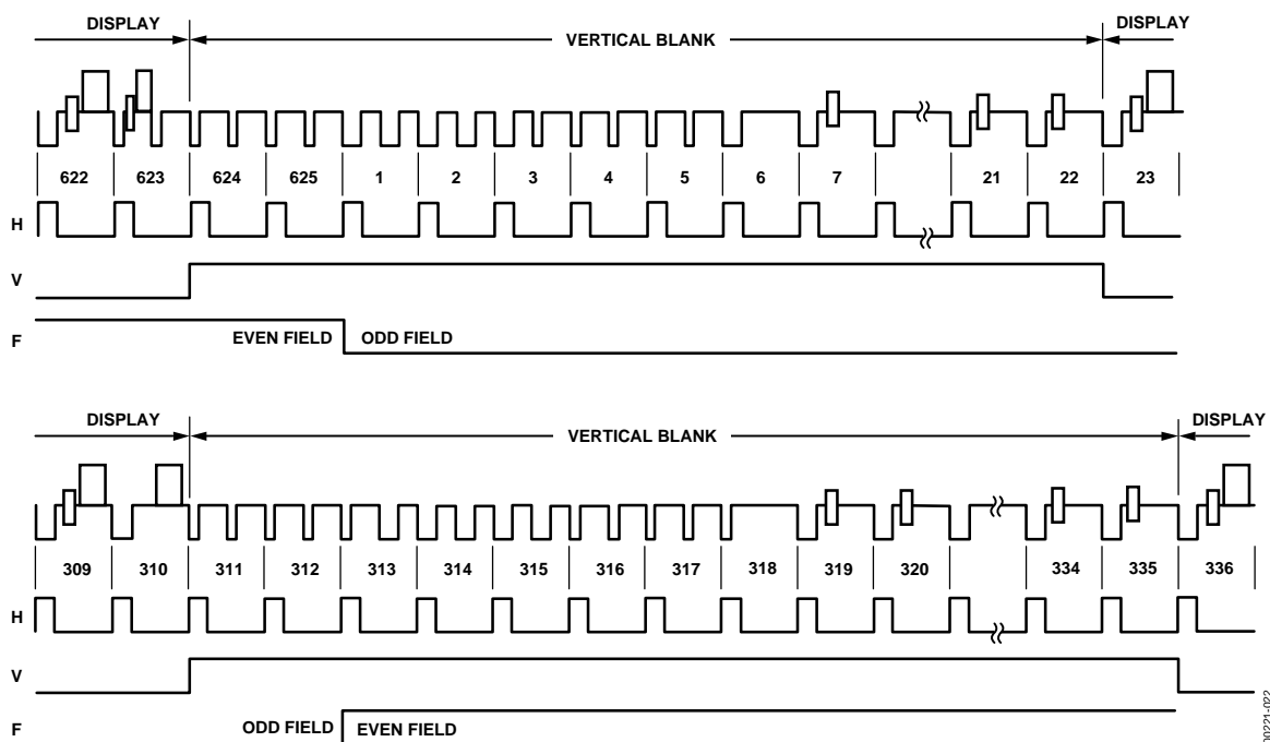
Figure 22. Timing Mode 0 (PAL Master Mode)
