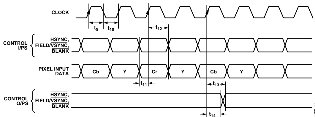
Figure 3. Pixel and Control Data Timing Diagram
