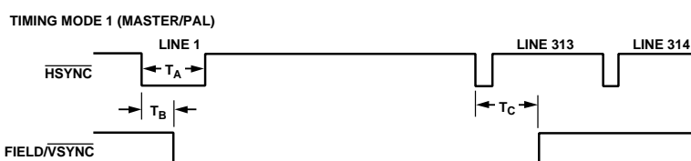
Figure 44. Timing Register 1
