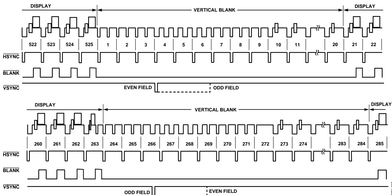
Figure 27. Timing Mode 2 (NTSC)
