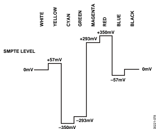
Figure 77. NTSC 100% Color Bars with Pedestal V Levels
