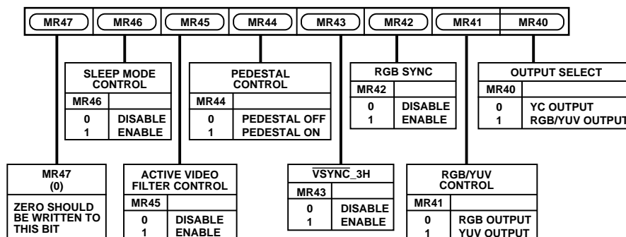
Figure 42. Mode Register 4
