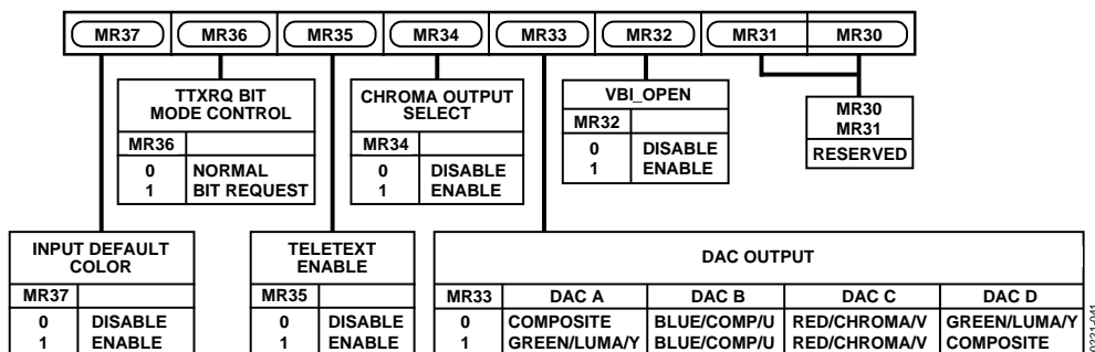
Figure 41. Mode Register 3
