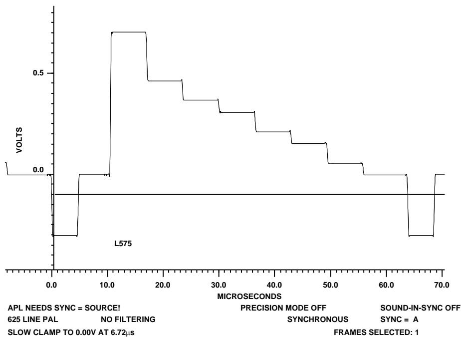
Figure 84. 100/0/75/0 PAL Color Bars Luminance
