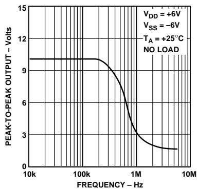
Maximum Output Voltage vs. Frequency
