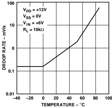
Droop Rate vs. Temperature
