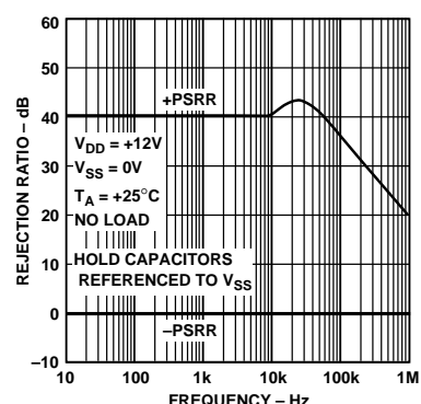
Hold Mode Power Supply Rejection
