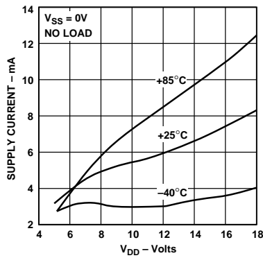
Supply Current vs. V_{DD}
