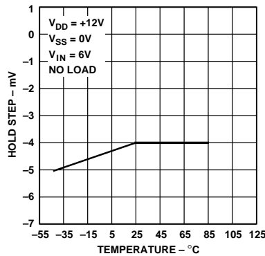
Hold Step vs. Temperature
