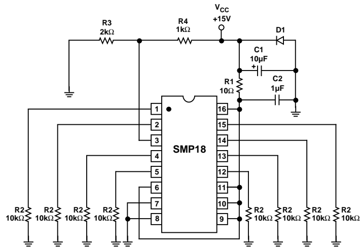
Burn-in Circuit
