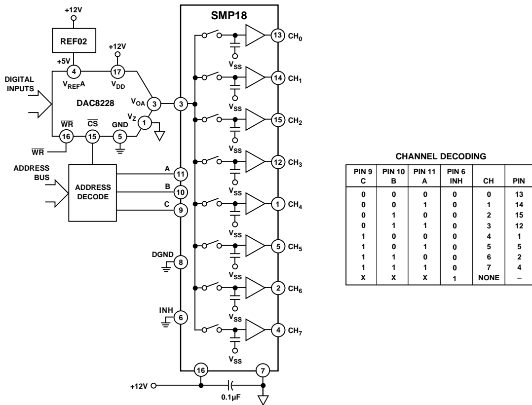
Figure 1. 8-Channel Multiplexed D/A Converter
