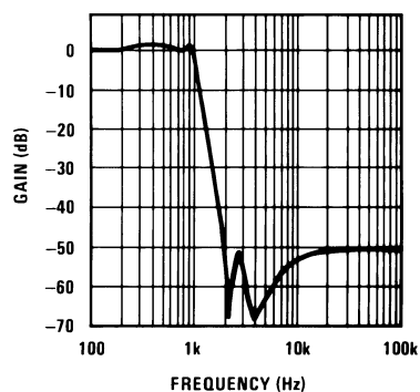
Figure 26. Lowpass Response
