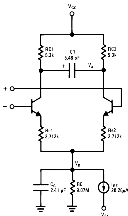
Figure 27. LM148, LM741 Macromodel for Computer Simulation
