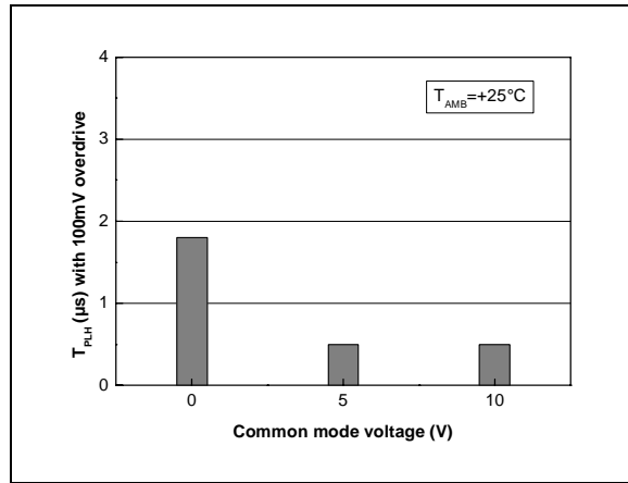
T_{PLH} vs V_{ICM} @ V_{CC}=5V and 100mV overdrive
