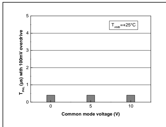
T_{PHL} vs V_{ICM} @ V_{CC}=10V and 100mV overdrive
