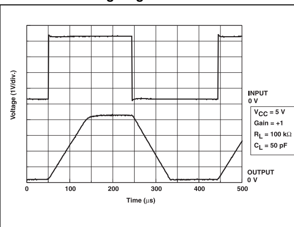
Figure 20. Slew rate vs. time for large input voltage signal
