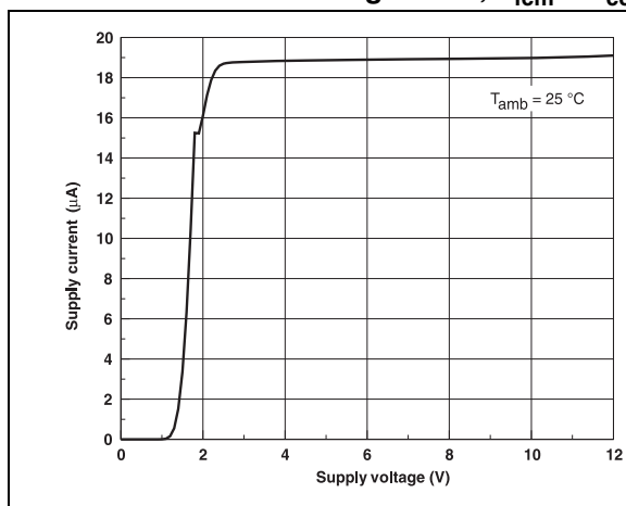
Figure 3. Supply current vs. supply voltage in follower configuration, V_{icm} = V_{CC}/2
