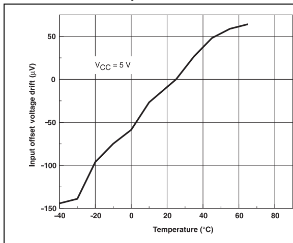
Figure 1. Input offset voltage vs. temperature
