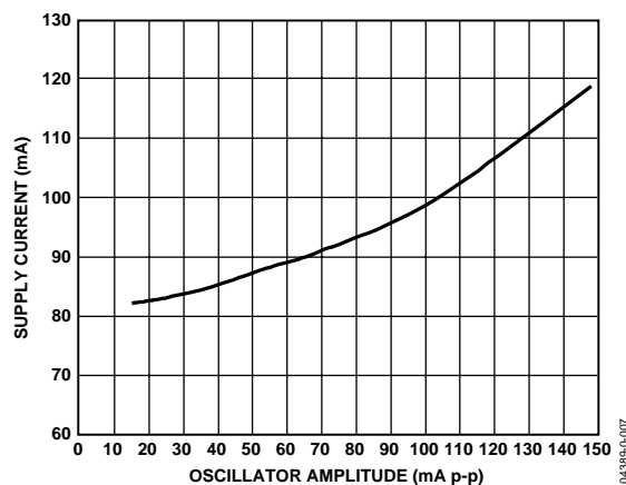
Figure 7. Supply Current vs. Oscillator Amplitude
