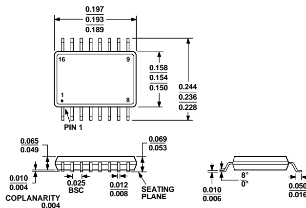
Figure 18.16-16-Lead Shrink Small Outline Package [QSOP] (RQ-16)
