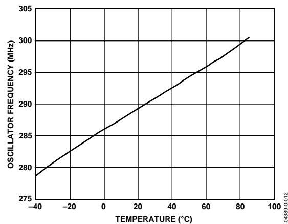
Figure 12. Oscillator Frequency vs. Temperature
