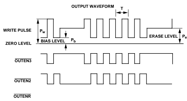
Figure 14. Typical Waveform
