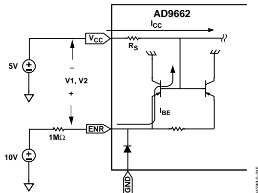
Figure 15. Junction Temperature Measurement Circuit
