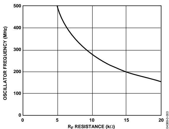
Figure 3. Oscillator Frequency vs. R_F
