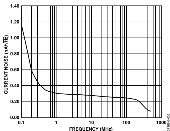
Figure 5. I_{OUR} Current Noise
