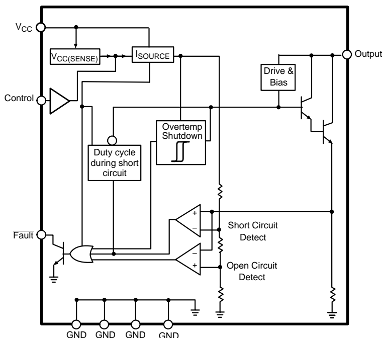
Figure 1. Block Diagram
