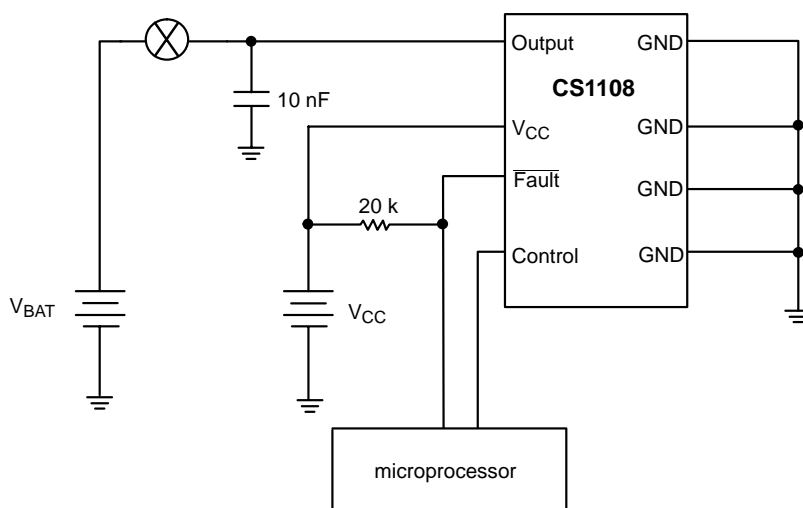
Figure 2. Applications Diagram
