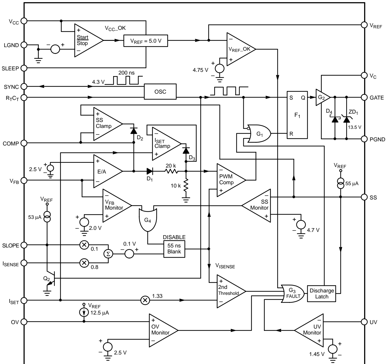
Figure 2. Block Diagram
