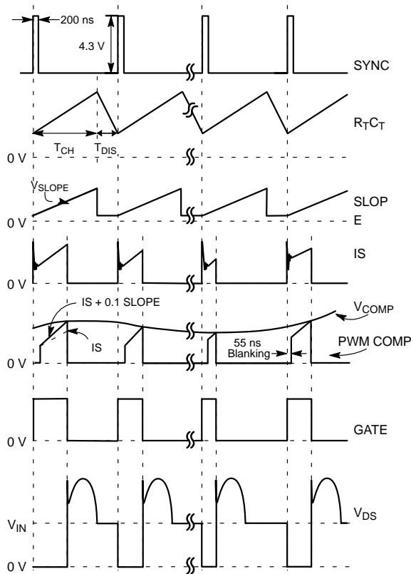
Figure 3. Typical Waveforms
