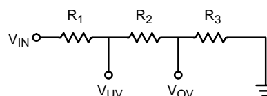
Figure 5. UV/OV Monitor Divider
