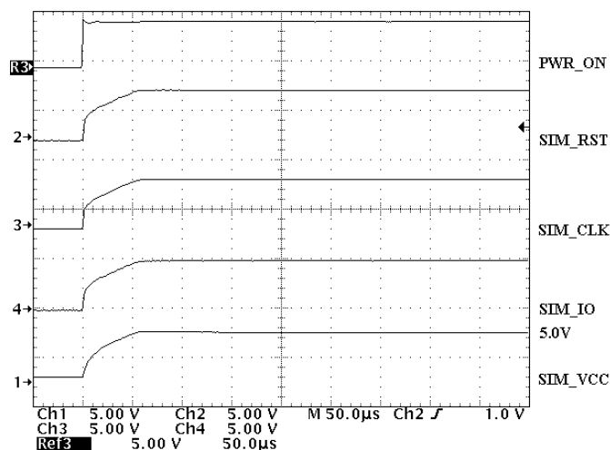
Figure 3. Power On Sequence
