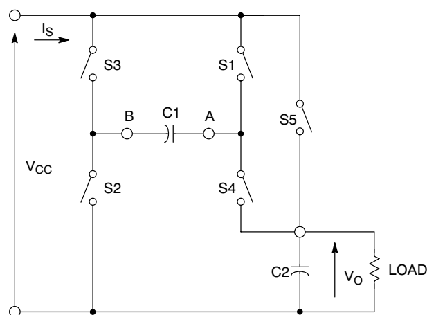
Figure 9. Basic Charge Pump Converter
