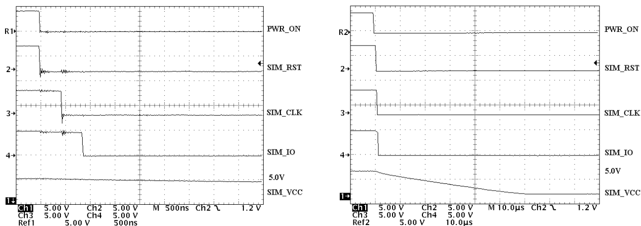
Figure 5. Power Down Sequence Oscilloscope
