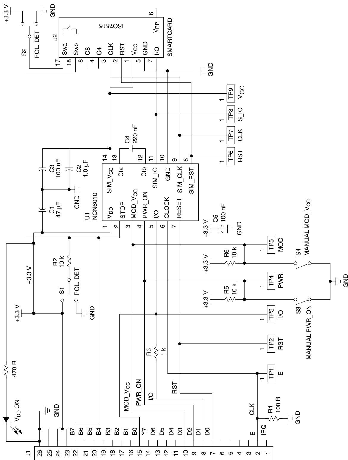
Figure 14. Engineering Test Board
