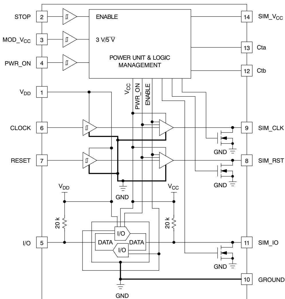
Figure 2. NCN6010 Block Diagram
