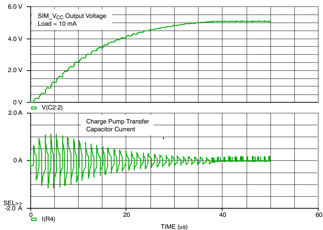
Figure 12. Simulated Charge Pump Typical Waveforms
