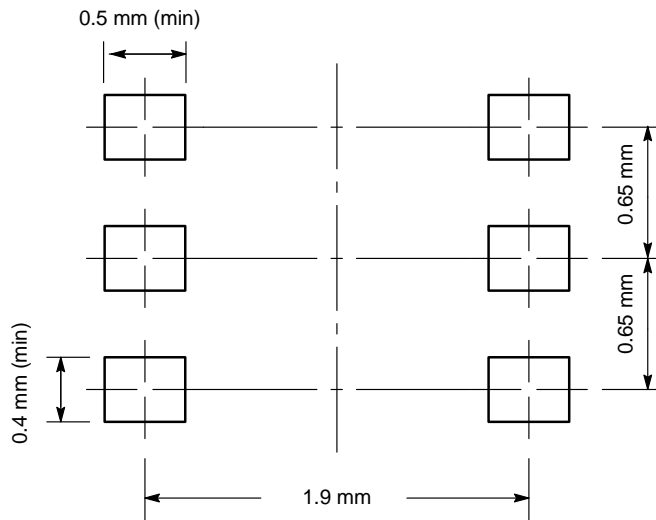
QFN 2x2.2
