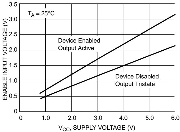
Figure 15. NCS2201/3 Enable Input Voltage versus Supply Voltage
