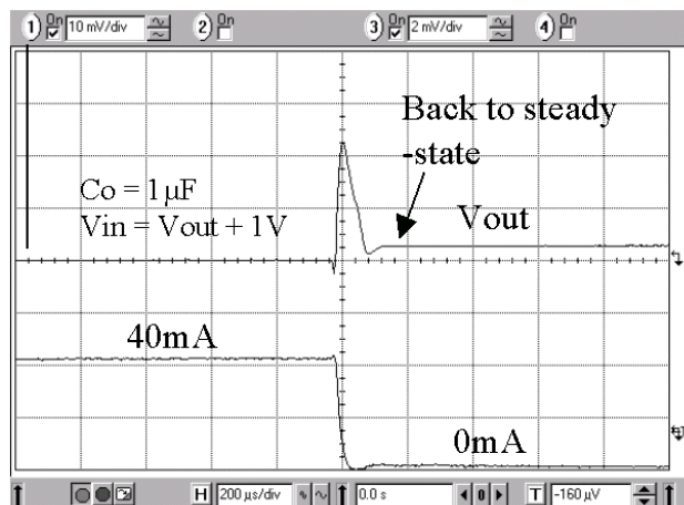
Figure 16. Load Transient Improvement Effect
