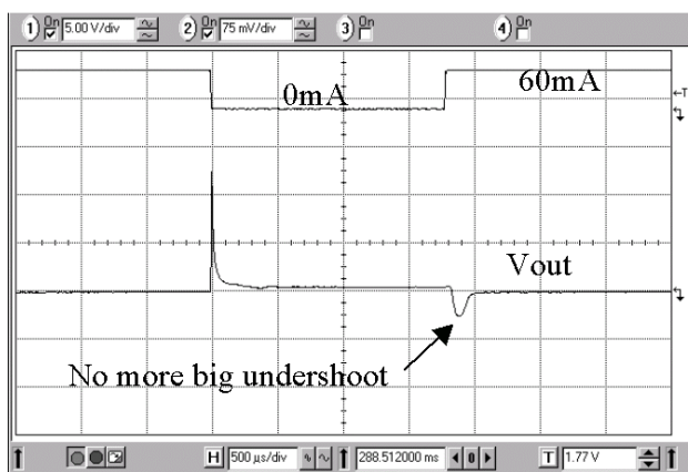
Figure 11. MC33762 with Load Transient Improvement
