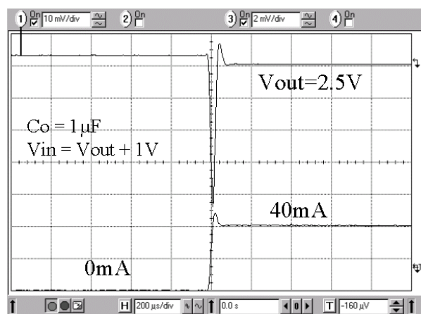
Figure 14. Discharge Effects from 0 to 40 mA
