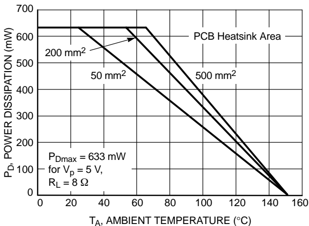
Figure 35. Power Derating – 9-Pin Flip-Chip CSP
