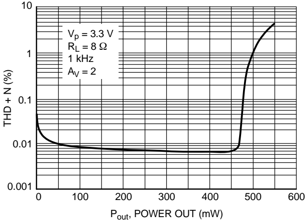
Figure 7. THD + N versus Power Out
