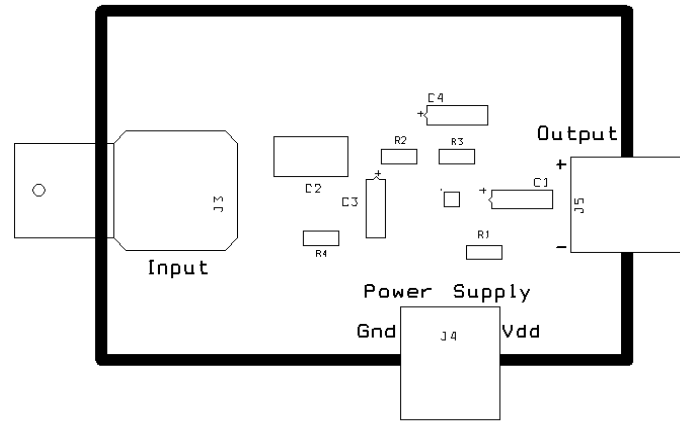
Silkscreen Layer
