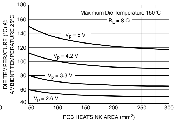
Figure 36. Maximum Die Temperature versus PCB Heatsink Area
