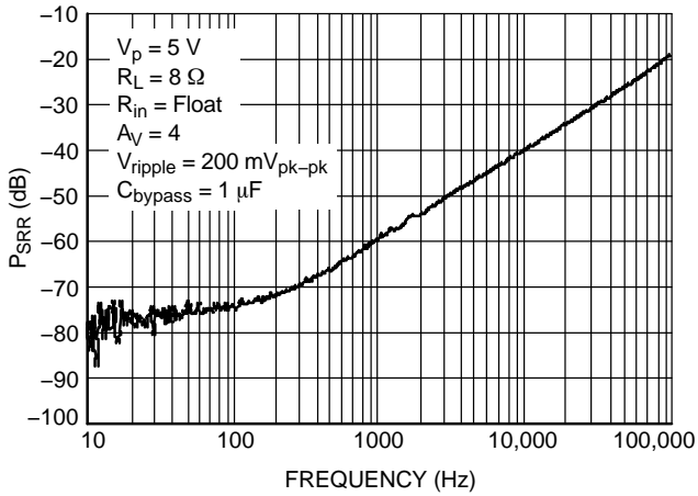
Figure 15. P SRR @ V p = 5 V
