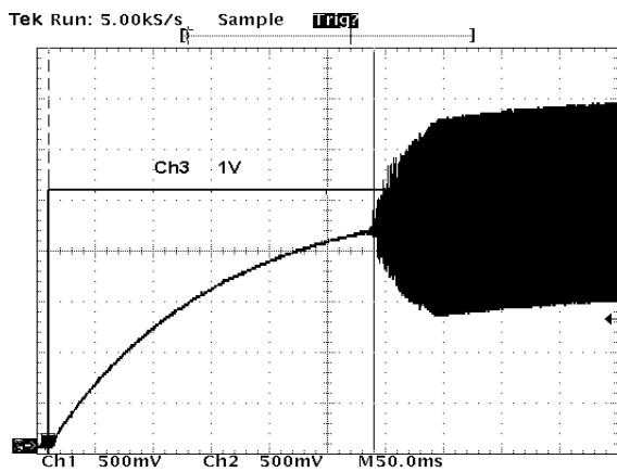
Figure 29. Turning On Time - V_p = 5 V
