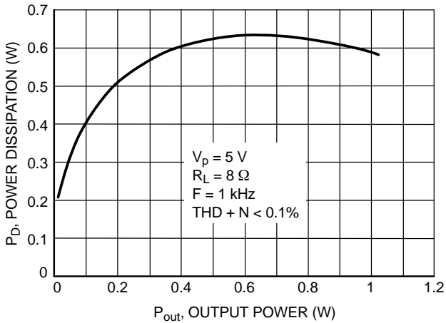
Figure 31. Power Dissipation versus Output Power
