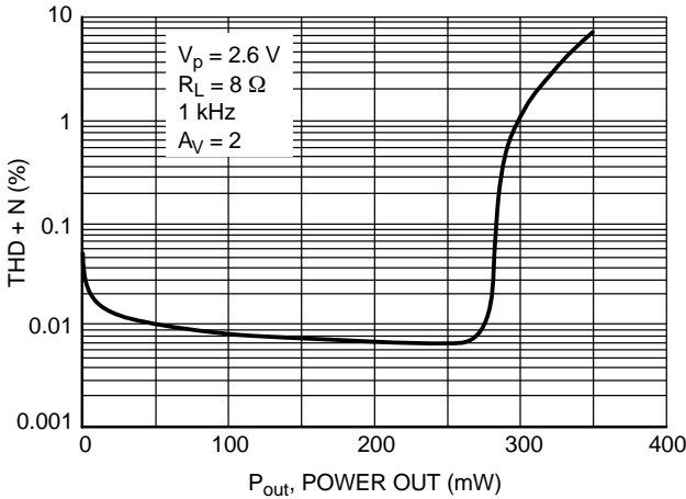
Figure 9. THD + N versus Power Out
