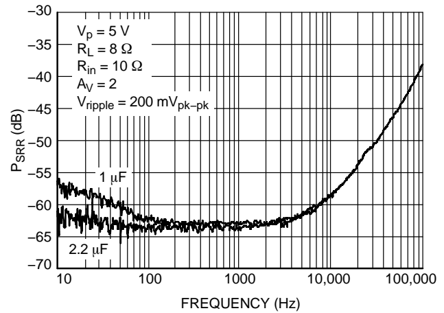
Figure 24. P SRR versus C bypass @ V p = 5 V
