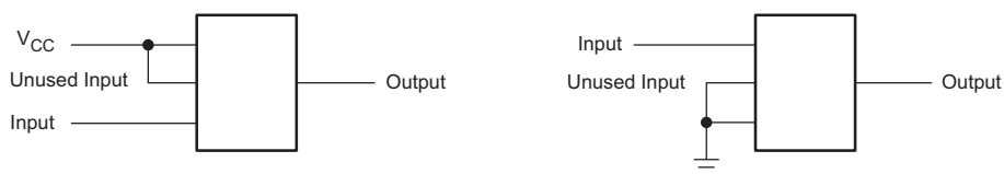
Figure 7. Layout Diagram
