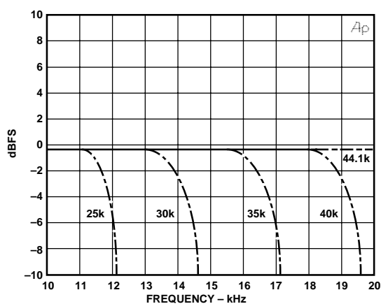
Figure 20. Digital Filter Signal Transfer Function, 10 kHz to 20 kHz, 44.1 kHz Input Sample Frequency, 44.1, 40, 35, 30 and 25 kHz Output Sample Frequencies
