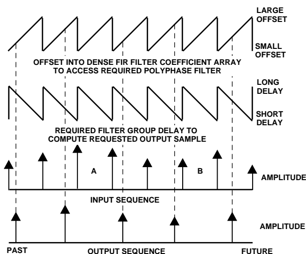
Figure 5. Input and Output Clock Event Relationship
