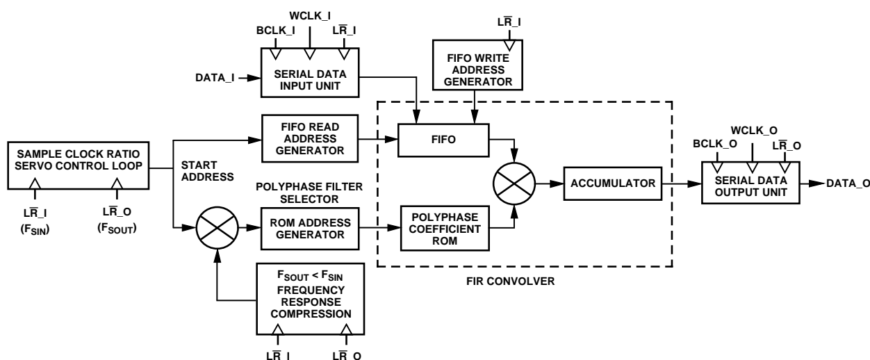
Figure 6. Functional Block Diagram
