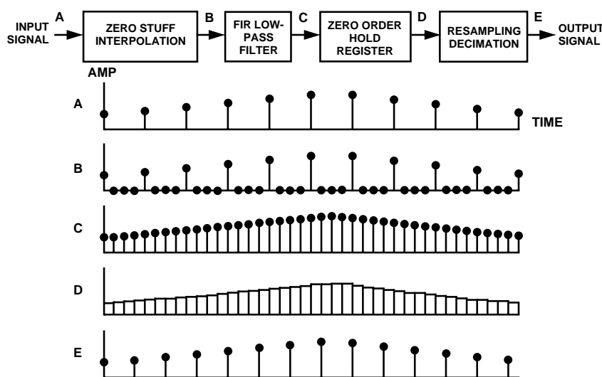
Figure 1. Interpolation/Decimation Model—Time Domain View
