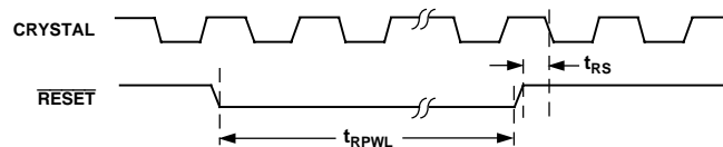
Figure 27. Reset Timing
