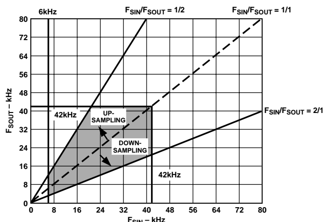
Figure 12. Allowable Input and Output Sample Frequencies F_{\text{CRYSTAL}} = 12 \text{ MHz} Case
