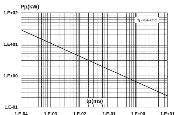
Fig. 1: Peak pulse power versus exponential pulse duration.
