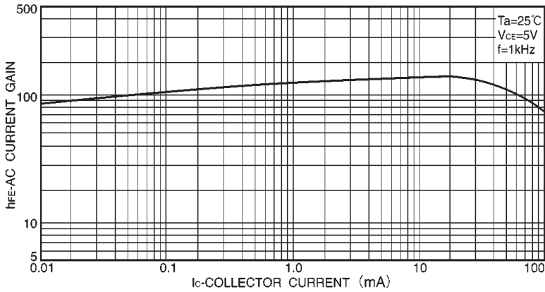
Fig.5 AC current gain vs. collector current
