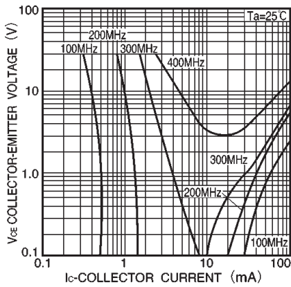
Fig.13 Gain bandwidth product
