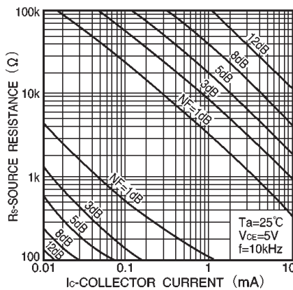
Fig.18 Noise characteristics ( II )
