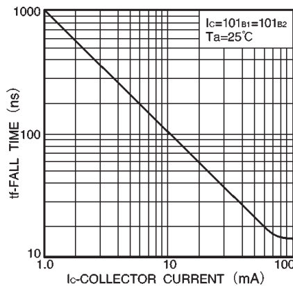
Fig.11 Fall time vs. collector current
