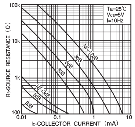
Fig.20 Noise characteristics ( IV )
