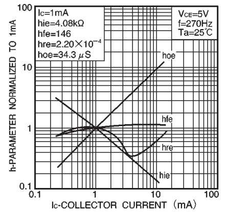
Fig.15 h parameter vs. collector current
