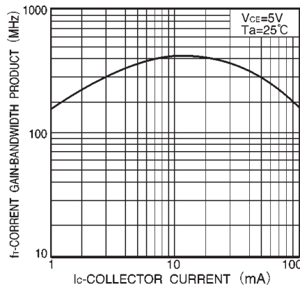
Fig.14 Gain bandwidth product vs. collector current
