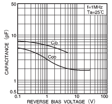
Fig.12 Input/output capacitance vs. voltage
