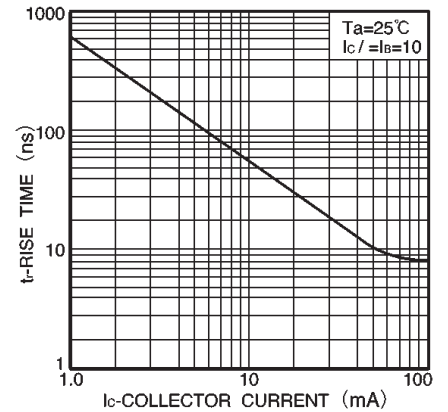
Fig.9 Rise time vs. collector current
