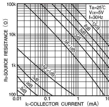
Fig.19 Noise characteristics ( III )
