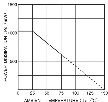
Fig.6 Temperature dependence of power dissipation curve (BA6286N)
