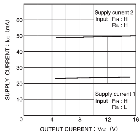
Fig.8 Supply current vs. output current
