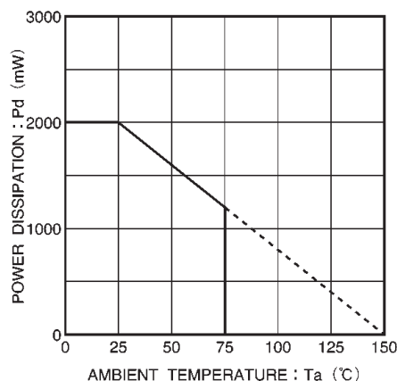
Fig.7 Temperature dependence of power dissipation curve (BA6286)
