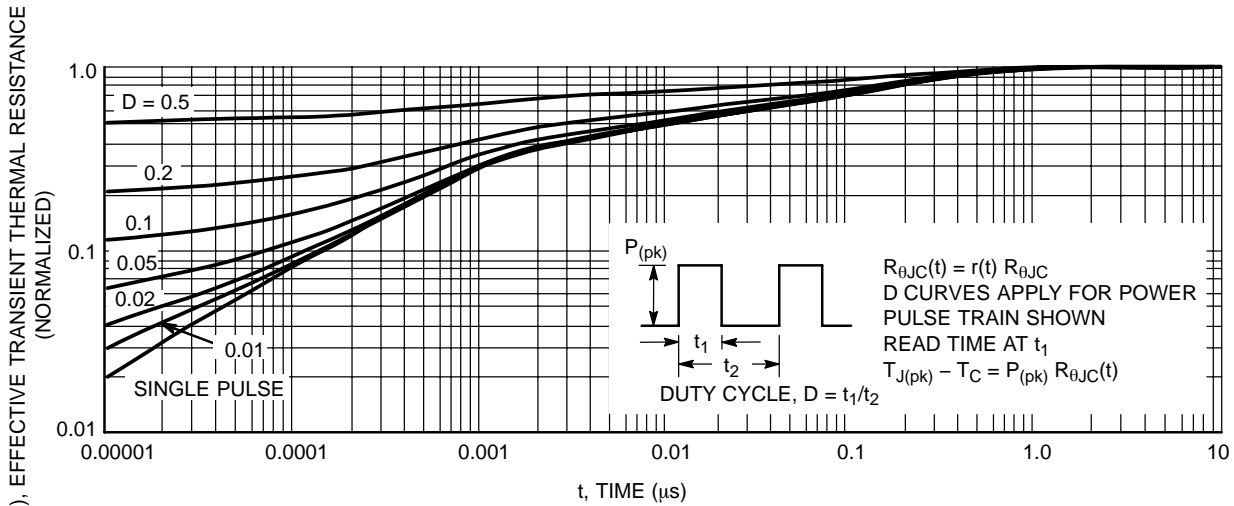
Figure 13. Thermal Response
