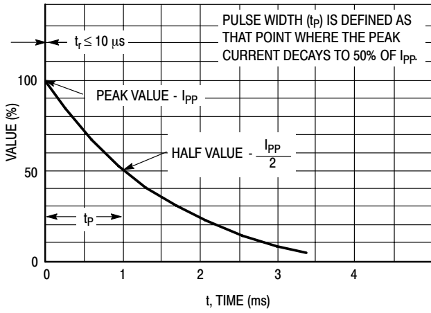
Figure 1. 10 × 1000 μs Pulse Waveform
