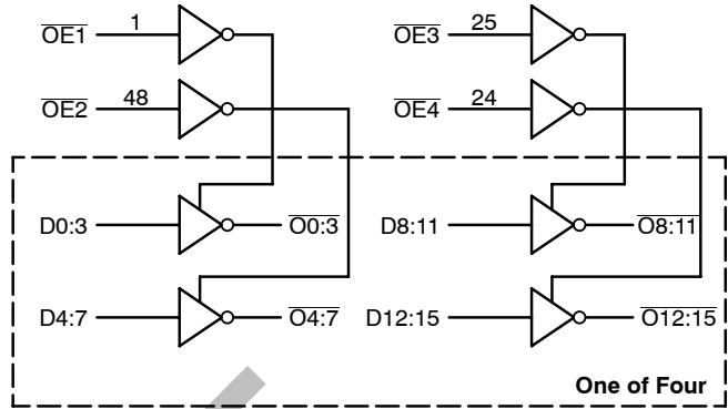
Figure 2. Logic Diagram
