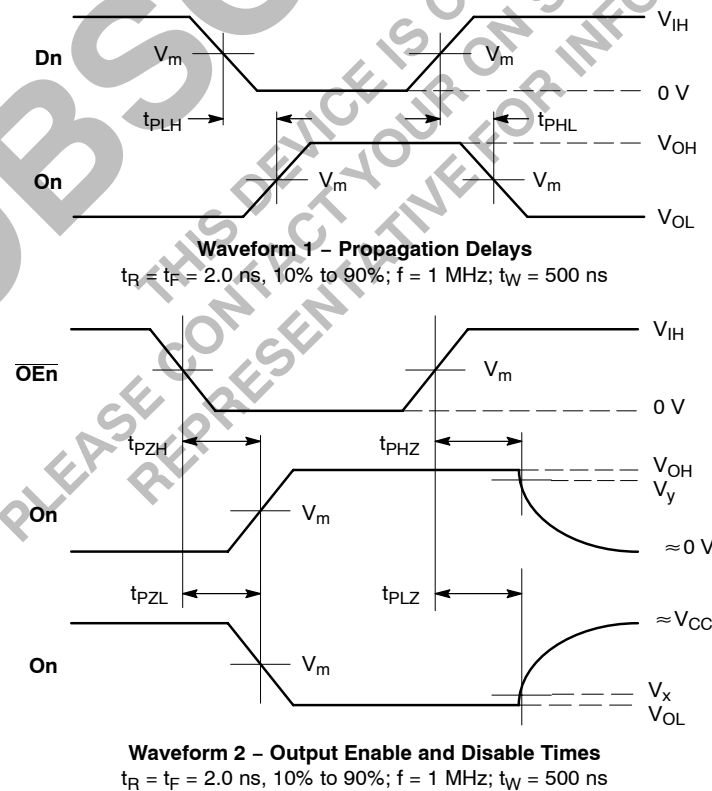
Figure 4. AC Waveforms
