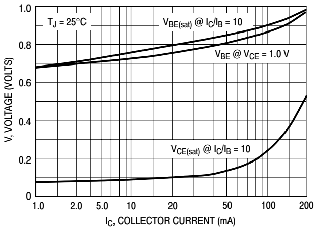
Figure 15. "ON" Voltages
