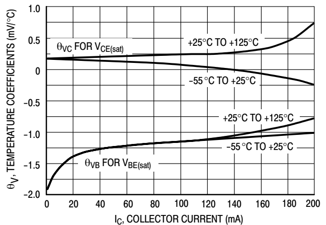
Figure 16. Temperature Coefficients
