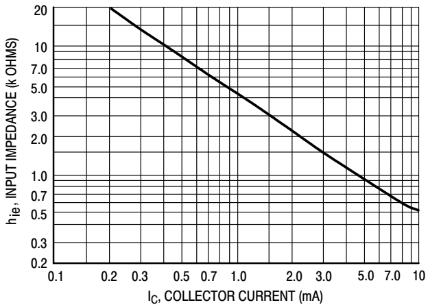
Figure 11. Input Impedance
