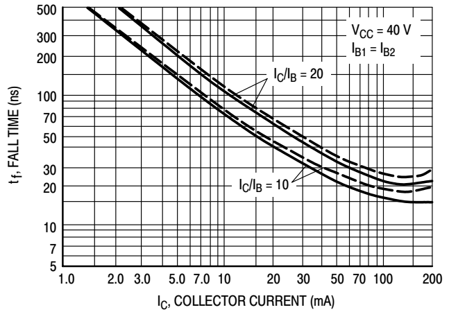
Figure 6. Fall Time
