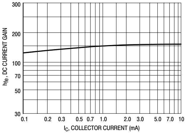
Figure 9. Current Gain
