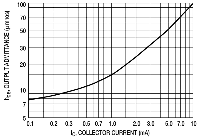
Figure 10. Output Admittance
