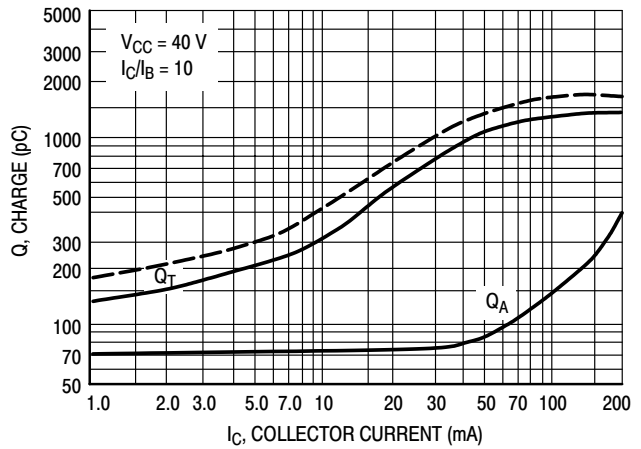
Figure 4. Charge Data
