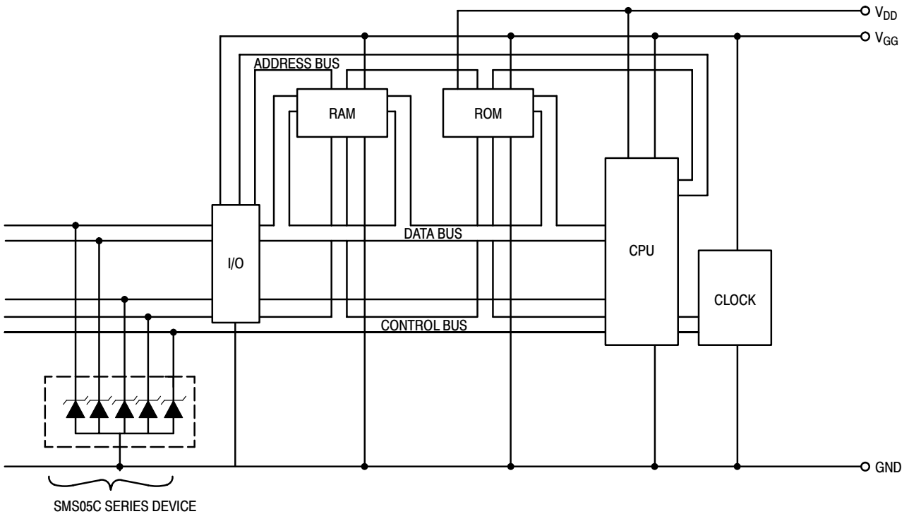
Figure 8. Microprocessor Protection
