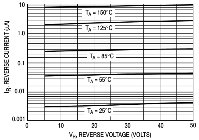
Figure 5. Leakage Current
