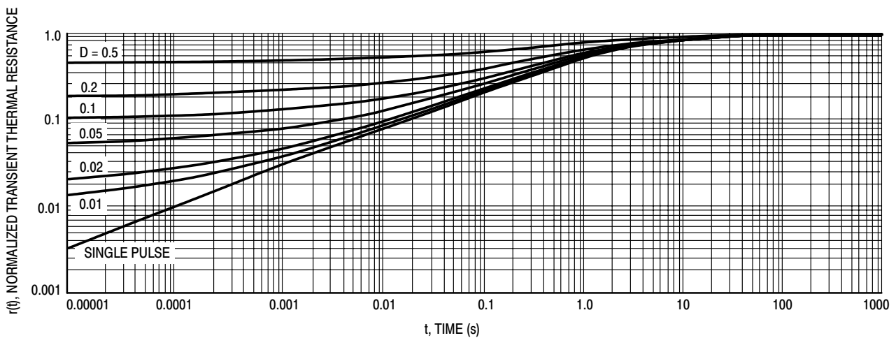
Figure 7. Normalized Thermal Response
