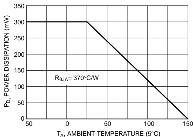
Figure 1. Derating Curve
